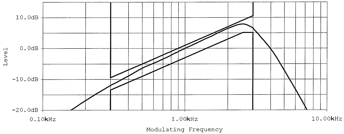
Frequency Response Test Frequency 156.800MHz (ch16)
