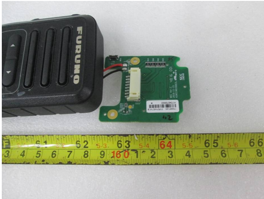
EUT (Handset 1) – Main Board Top View
