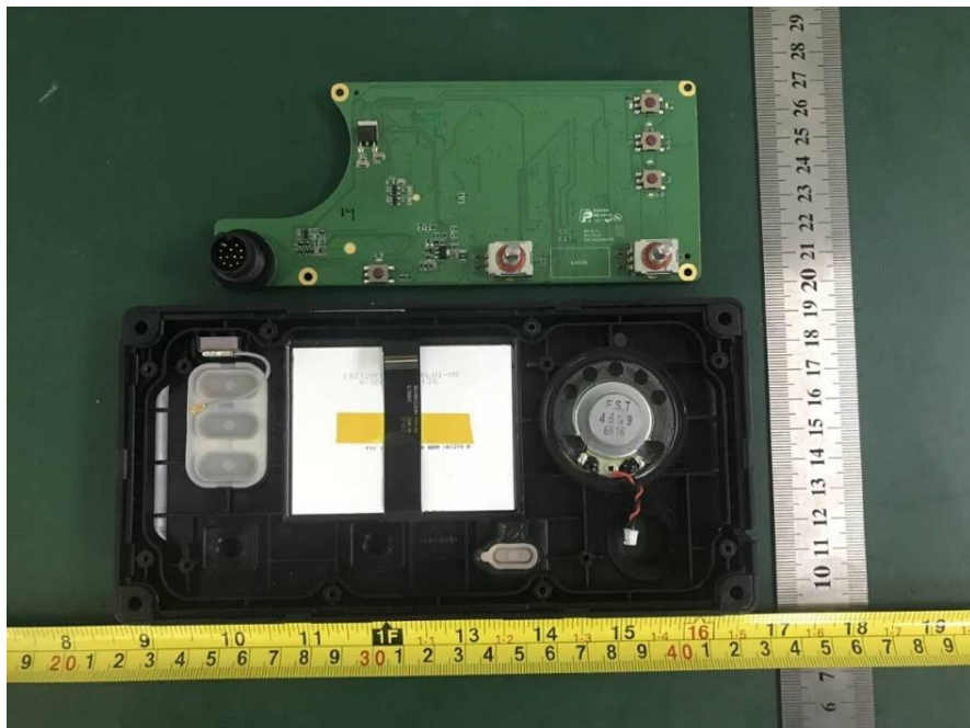
EUT (Handset 2) – Cover off View 2
