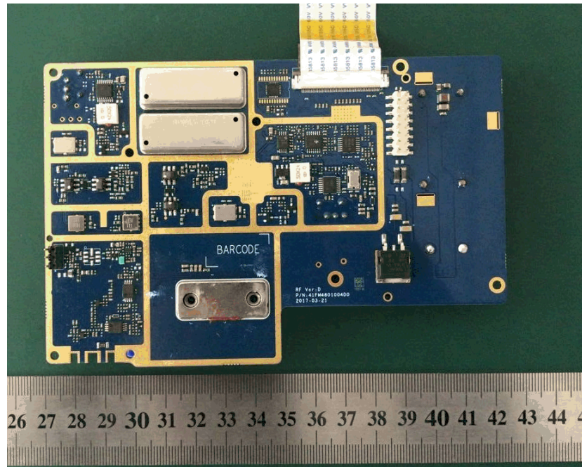
EUT- Main Board 1 Top View
