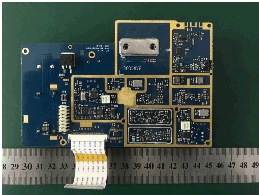
EUT- Main Board 1 Shielding off Top View
