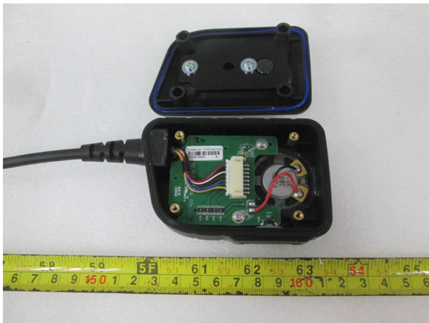
EUT (Handset 1) – Cover off View
