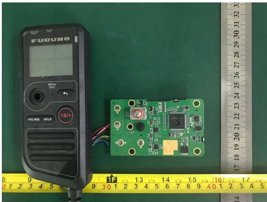
EUT (Handset 2) – Main Board Bottom View
