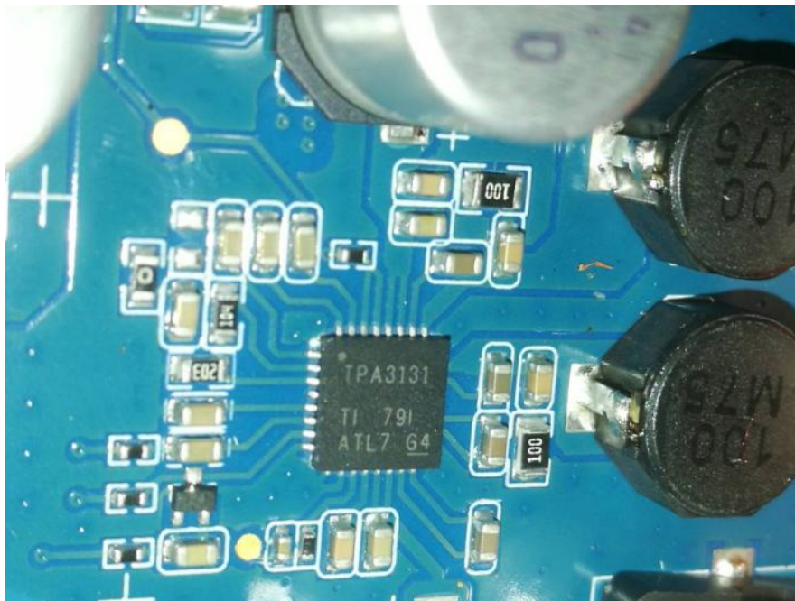
EUT – IC Chip 11 View
