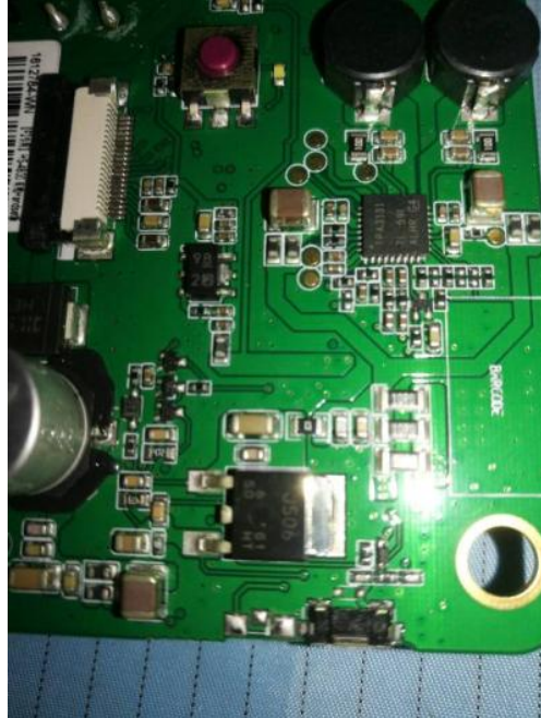
EUT (Handset) –IC Chip View 1
