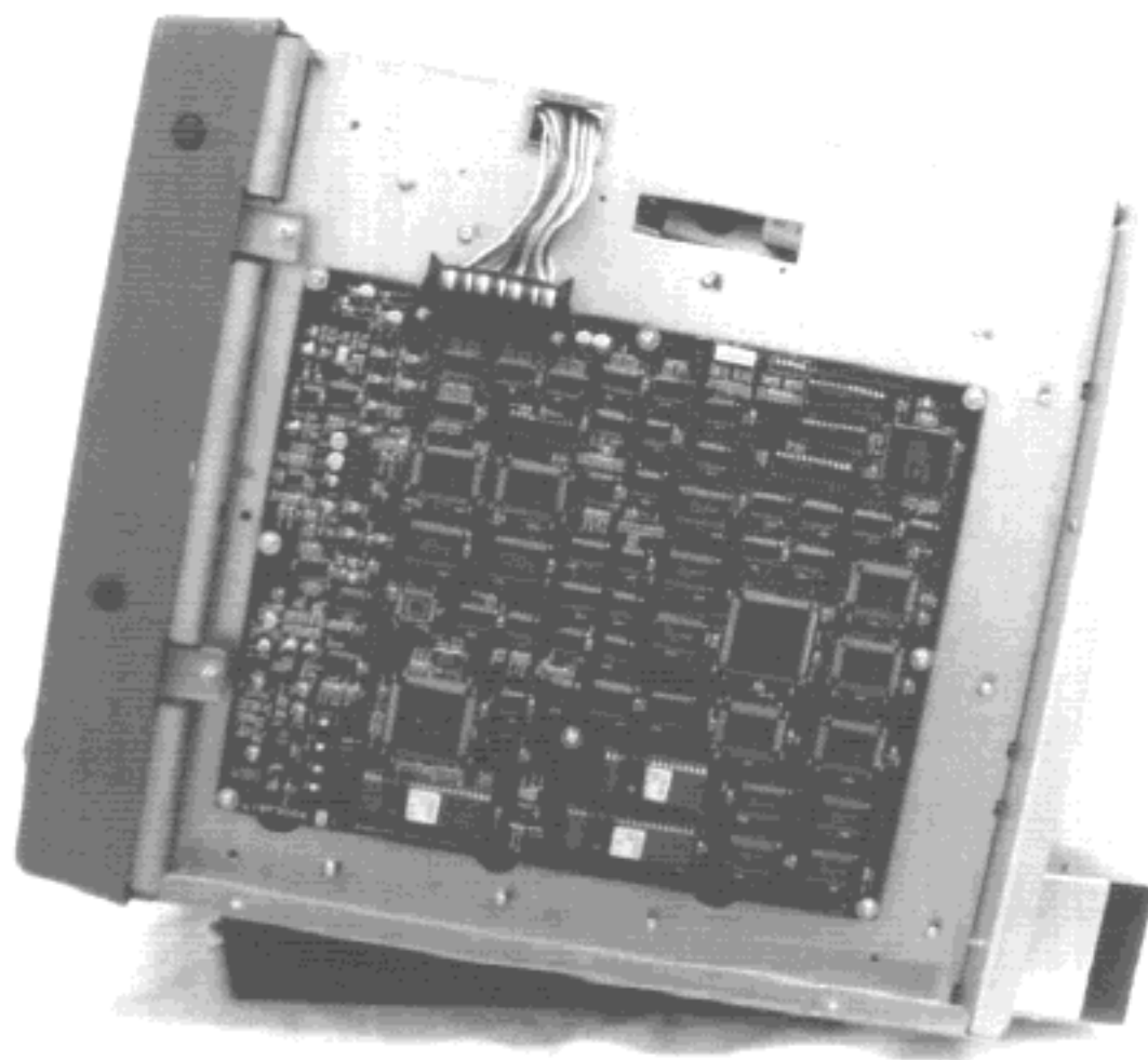
Photo 10.3 Display Unit (RDP-119) Right Side View (cover removed) (showing ARP-17 (18P9004, option) Board)
