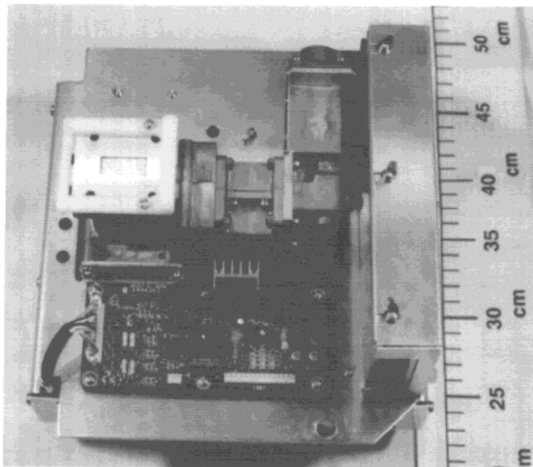
Photo 10.9 Transceiver Module Top View (showing Circulator, Limiter & RFC board (03P9243))
