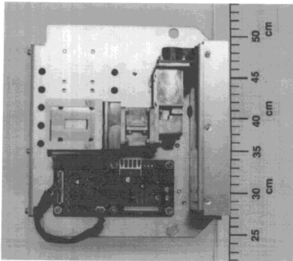
Photo 10.9 Transceiver Module Top View (showing Circulator, Limiter & RFC board (03P9243))
