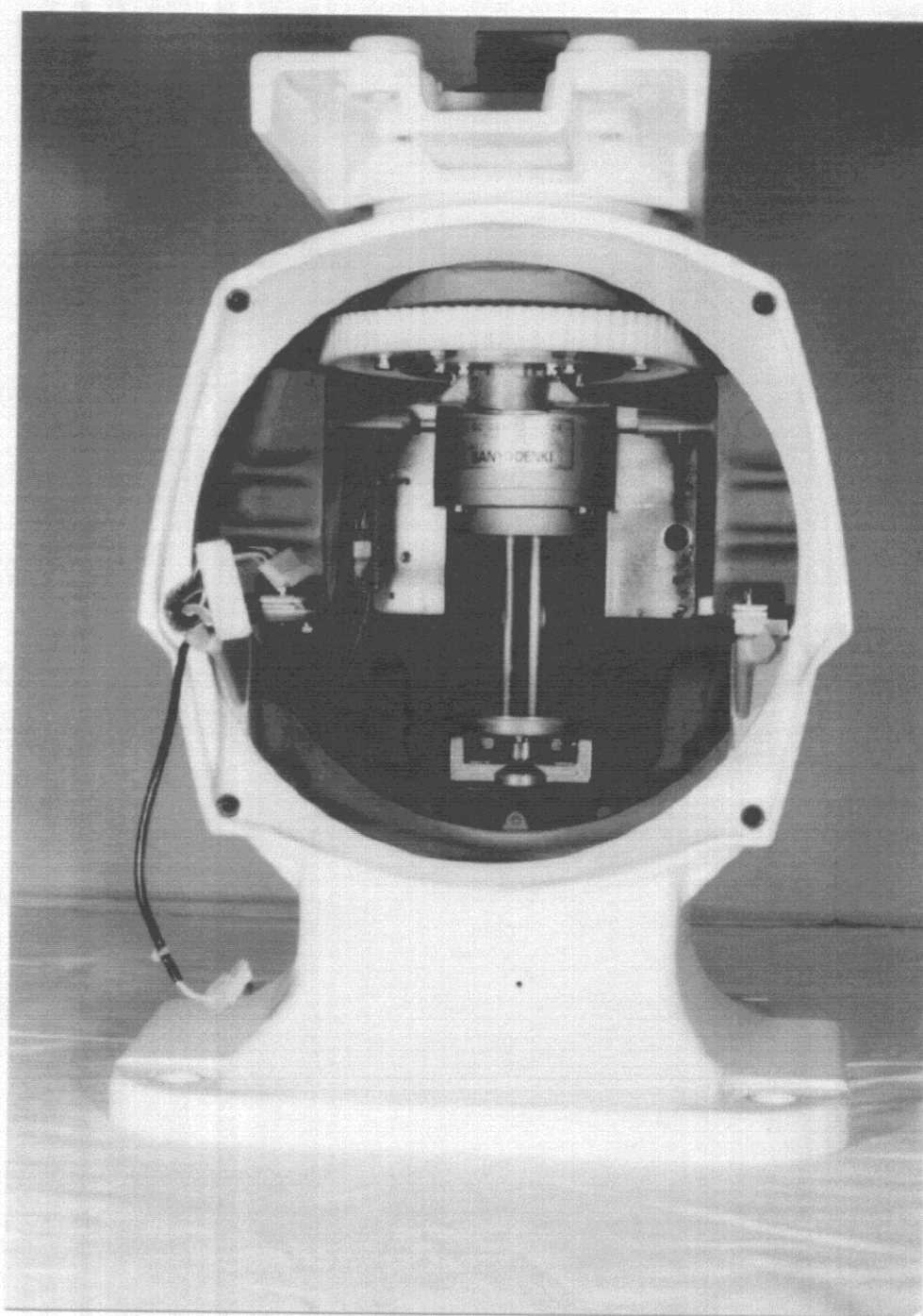
Photo 10.7 Scanner Unit Inside View (Transceiver Module removed)
