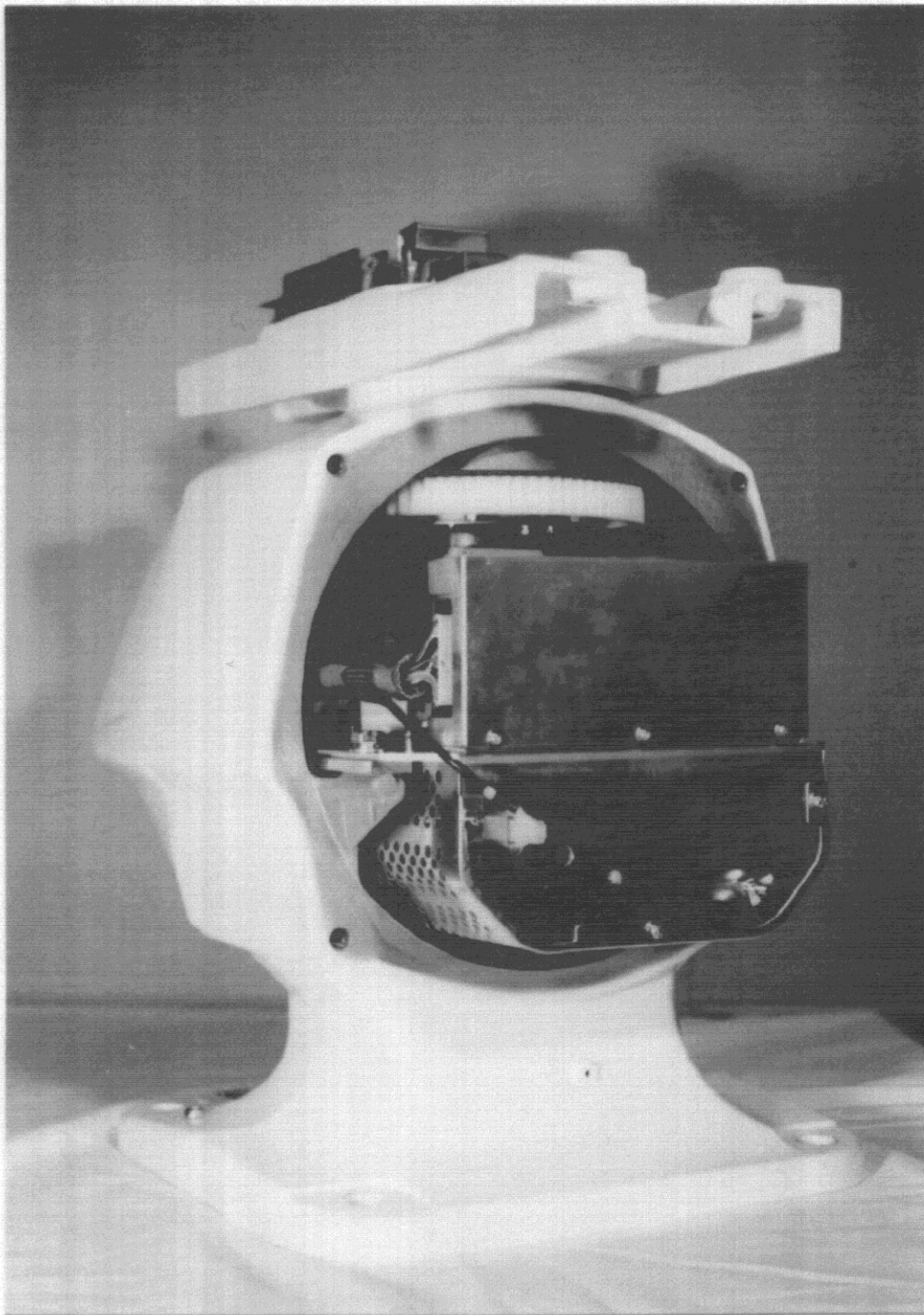
Photo 10.6 Scanner Unit Inside View (cover removed) (showing Transceiver Module)
