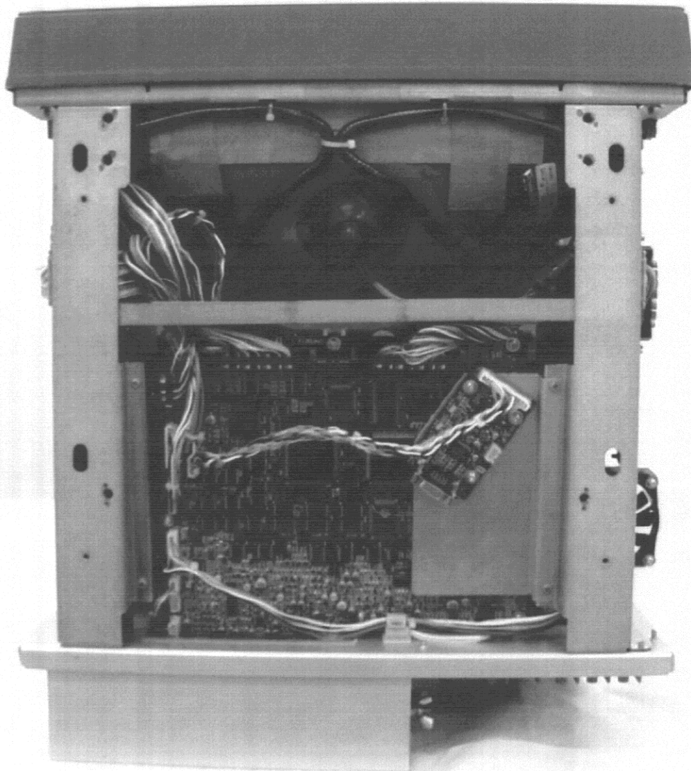
Photo 10.2 Display Unit (RDP-119) Top View (cover removed) (showing CRT, SPU Board (03P9230) and Video Interface (03P9229, option))
