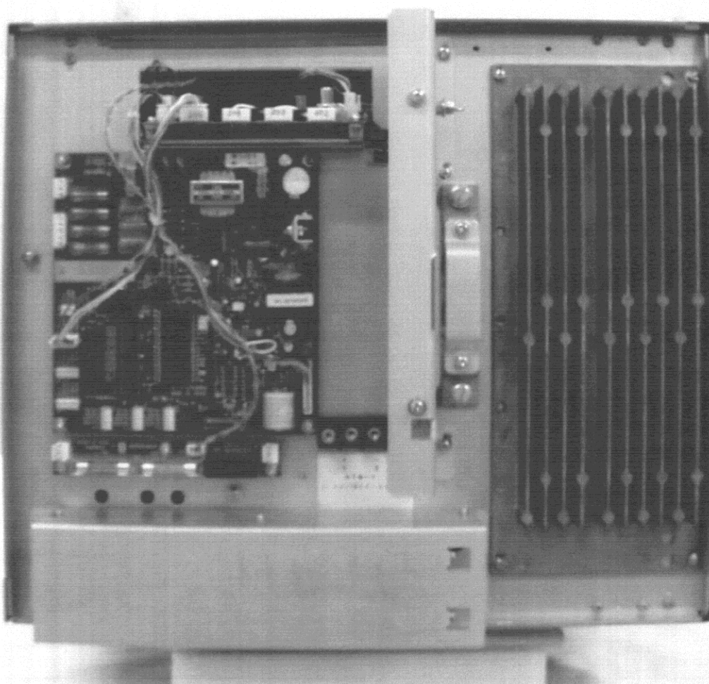
Photo 10.5 Display Unit (RDP-119) Rear View (cover removed) (showing GYRO CONVERTER (64P1106, option) Board)
