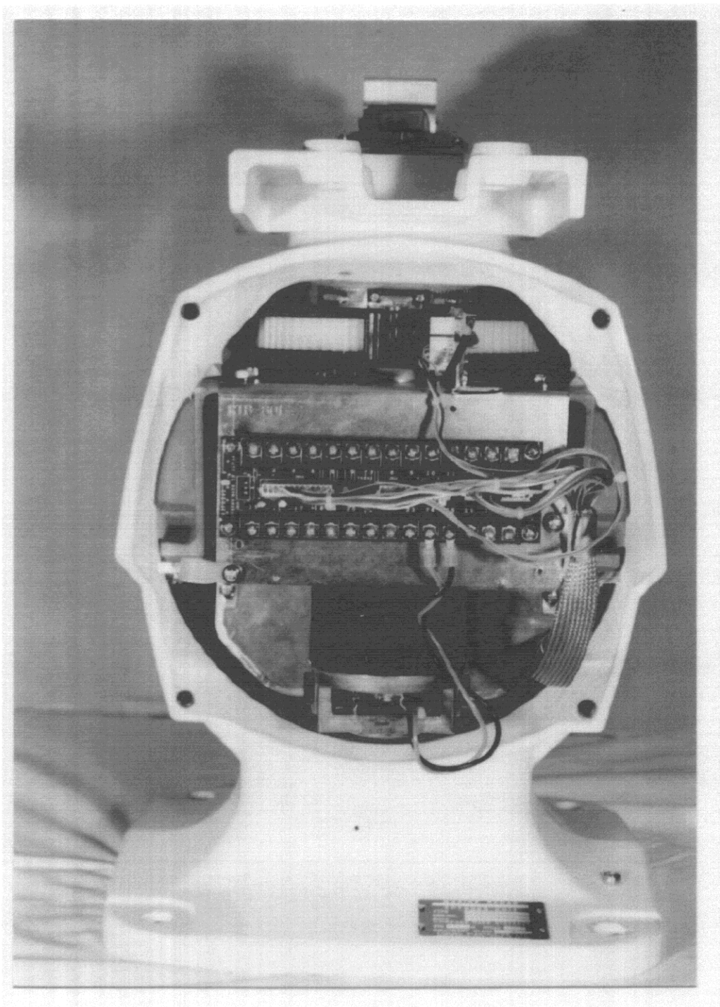
Photo 10.8 Scanner Unit Inside View (cover removed) (showing TB Board (03P9242))
