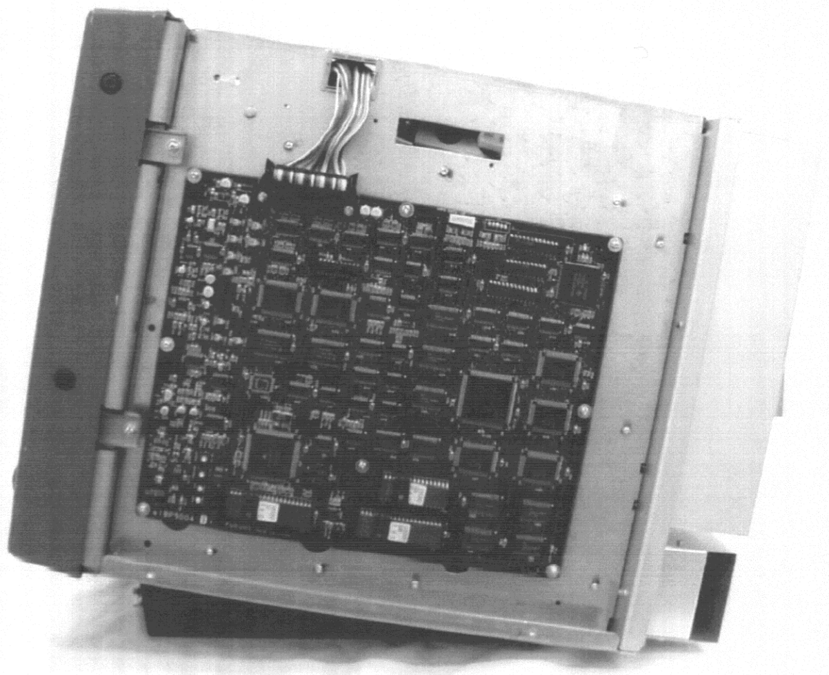
Photo 10.3 Display Unit (RDP-119) Right Side View (cover removed) (showing ARP-17 (18P9004, option) Board)
