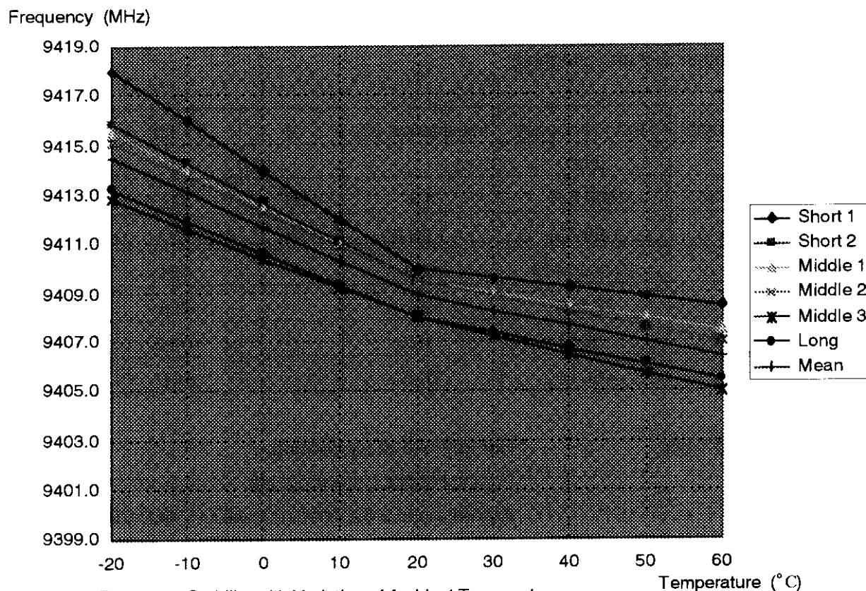
Fig.8.2 Frequency Stability with Variation of Ambient Temperature
