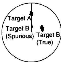
Figure 3-3 Sidelobe echoes
