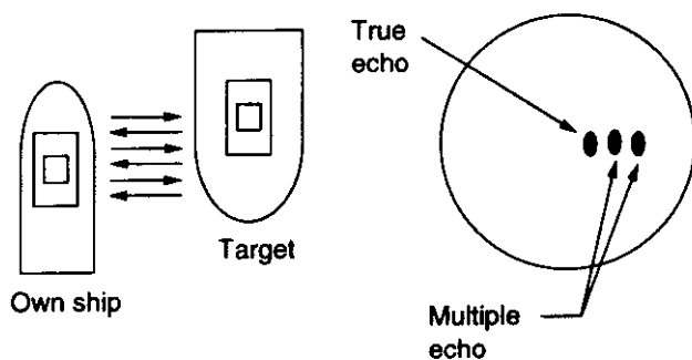
Figure 3-4 Virtual image
