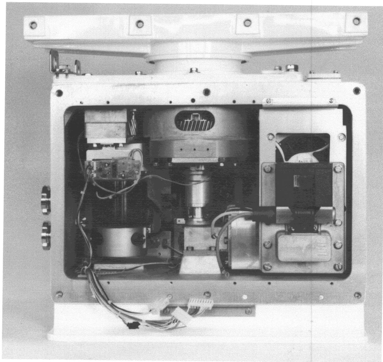
Photo 10.9 Scanner Unit Inside View (cover and RF Module removed) (showing Scanner Motor, Gear-box and Magnetron)
