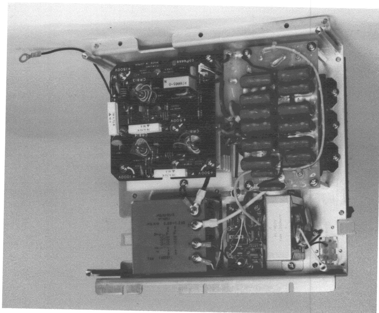
Photo 10.10 RF Module Inside View (showing Pulse Transformer, MD (03P6668) and PFN (03P6669) boards)
