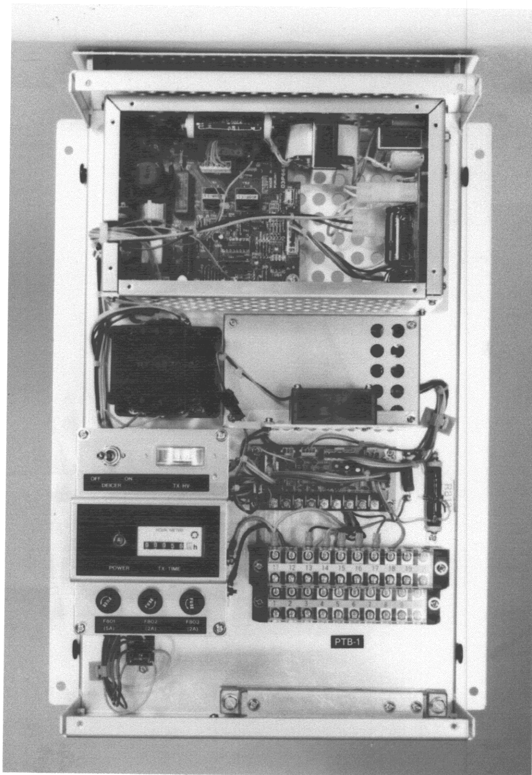
Photo 10.6 Power Supply Unit (PSU-002) Inside View (cover removed) (showing TX-HV and Power supply modules, Power Transformer and Terminal boards)
