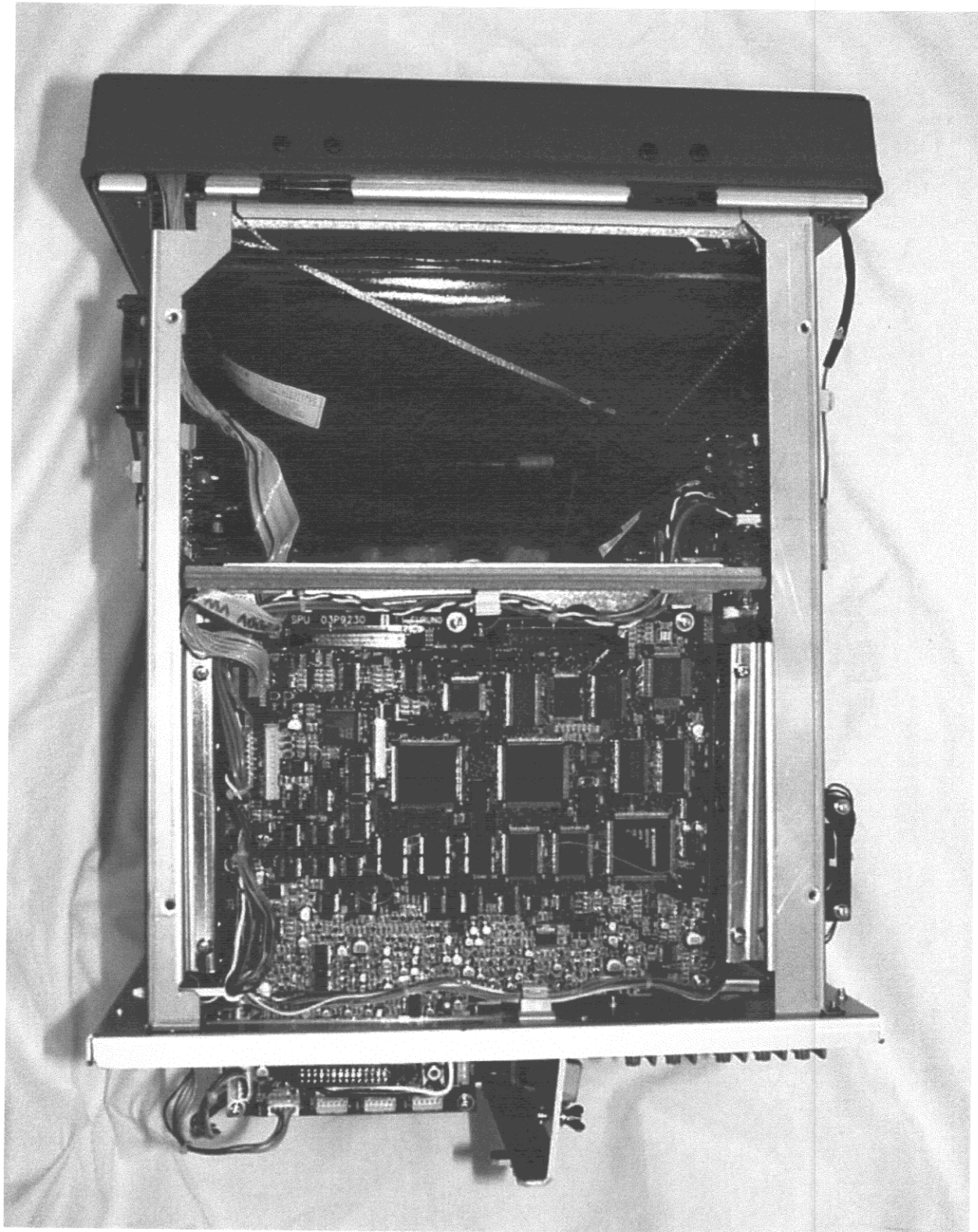
Photo 10.2 Display Unit (RDP-120) Top View (cover removed) (showing CRT and SPU Board (03P9230))
