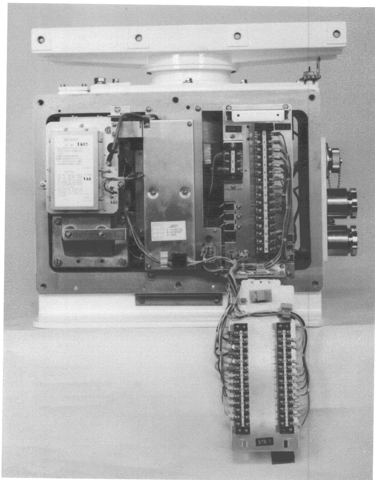
Photo 10.7 Scanner Unit (RSB-0051) Inside View (cover removed) (showing MIC, IF AMP. and Terminal boards)
