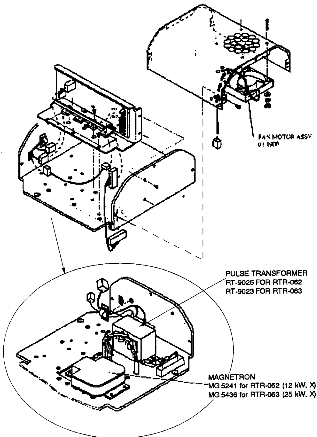
RF MODULE, BOTTOM VIEW
