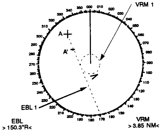
(a) Evaluating the target ship course and CPA in relative motion mode
