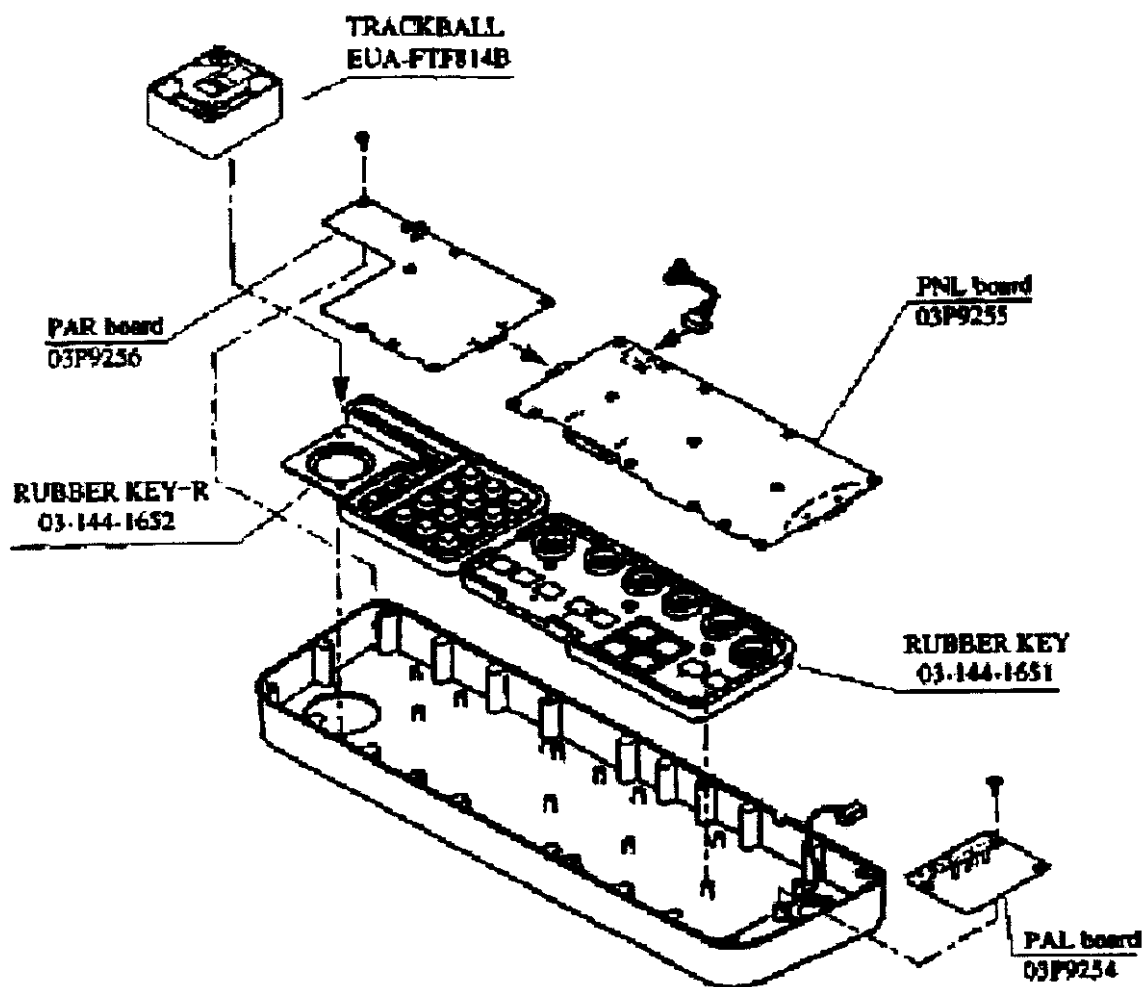
EXPLODED VIEW OF DISPLAY UNIT CONTROL HEAD
