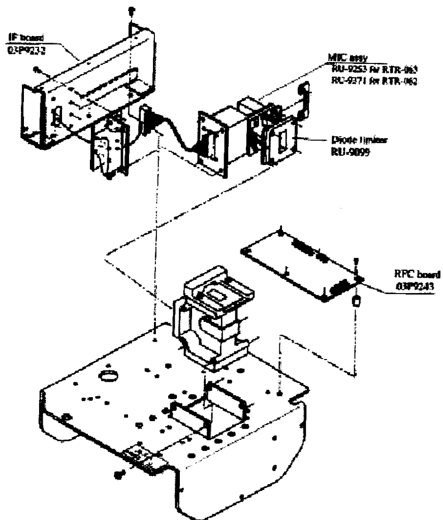
RF module, top view
