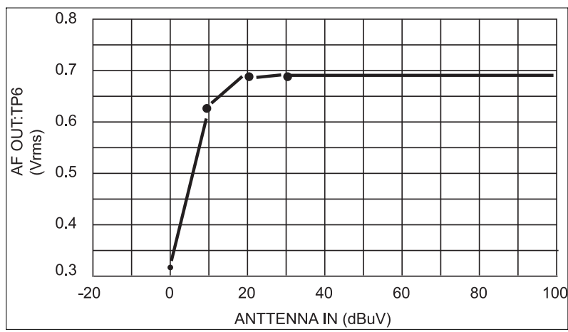
Fig.6.2.3.1-14 Input vs. output on W/R Board
