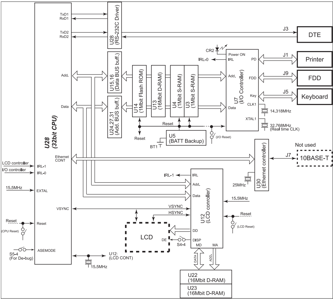
Fig.6.2.3.4-2 Block diagram of TERM CPU Board
