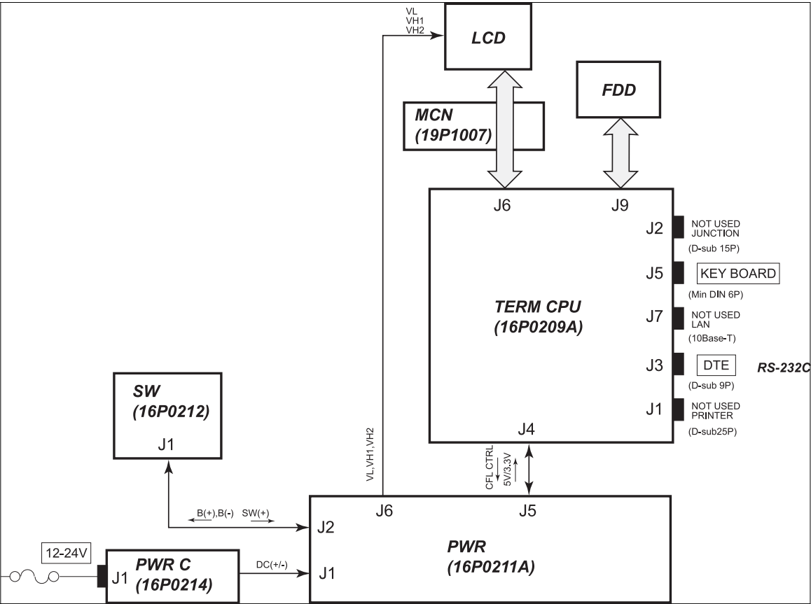
Fig.6.2.2.3-1 Block diagram of IB-583
