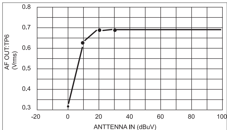
Fig.6.2.3.1-16 Input vs. output on W/R Board
