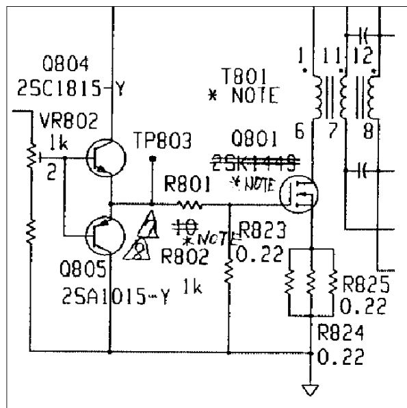
Fig. 3.2.1.2 Test Point for Trigger Pulse (in MD board (MD9052) of Radar Antenna Unit)
