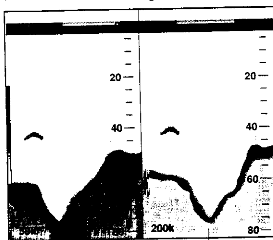
Figure 4-6 Dual-frequency display
