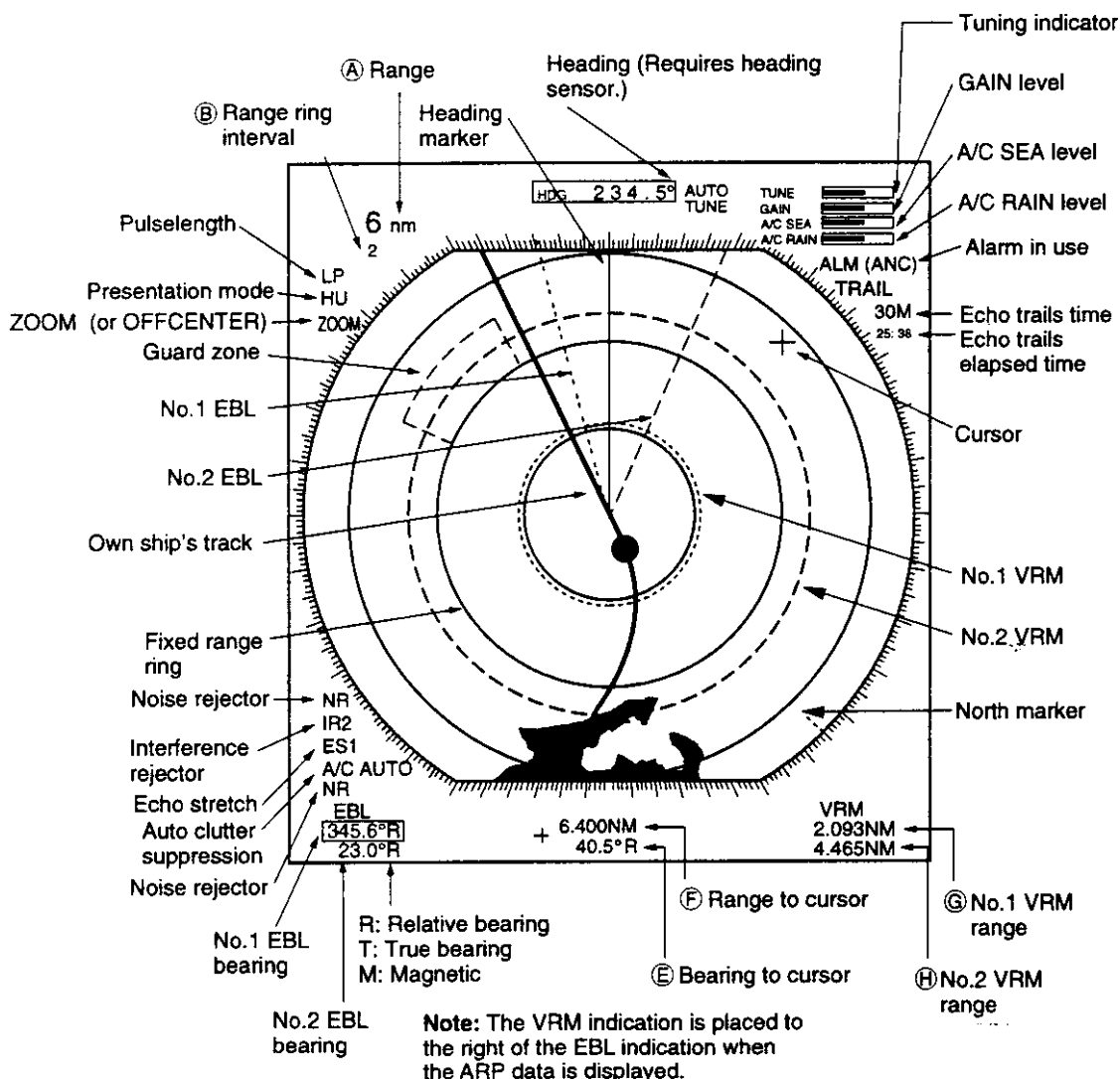
Figure 1-9 Radar display
