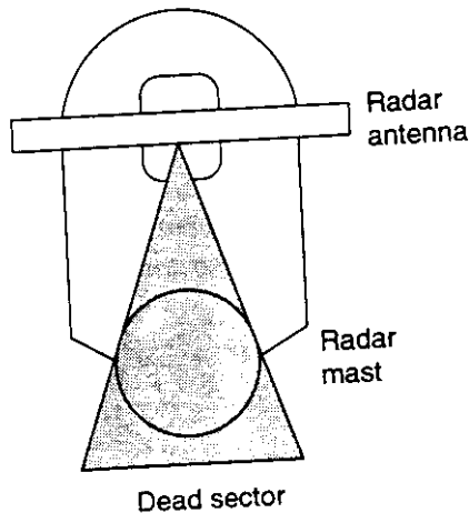
Figure 2-31 Dead sector
