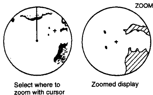
Figure 2-22 Zoom feature
