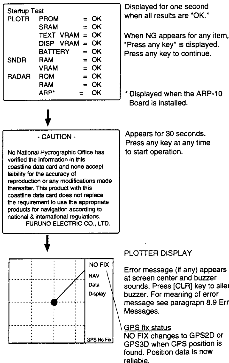
Figure 1-7 Start-up sequence
