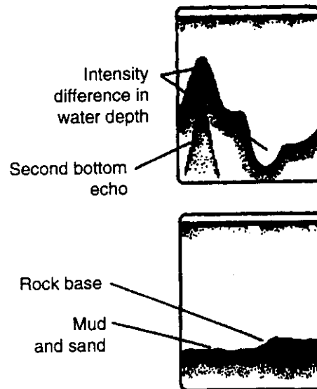
Figure 4-22 Bottom echoes
