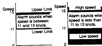
Figure 3-35 How the speed alarm works
