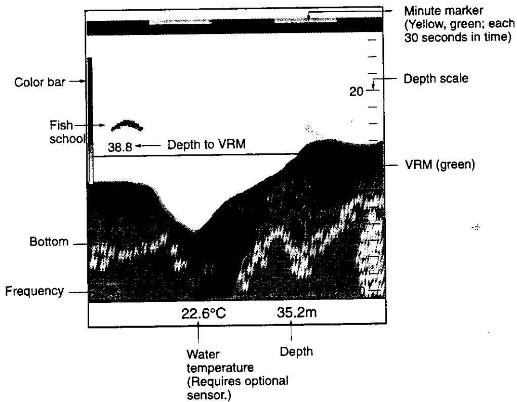
Figure 1-12 Sounder display
