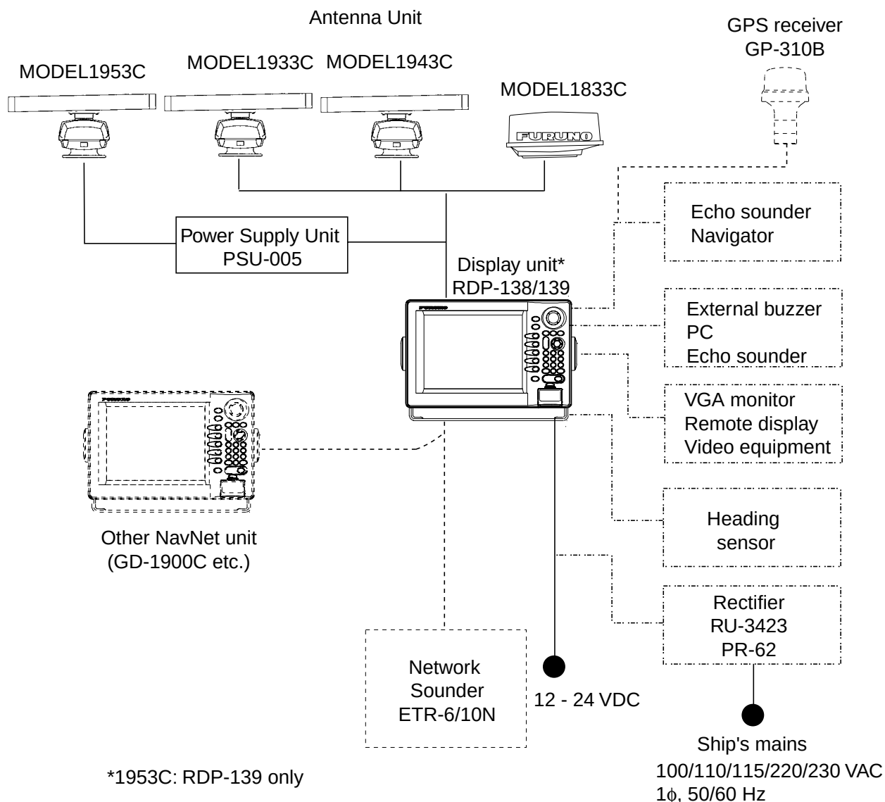
NavNet system (Model 1833C/1933C/1943C/1953C)
