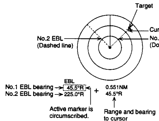
Figure 2-11 How to measure bearing with the EBL
