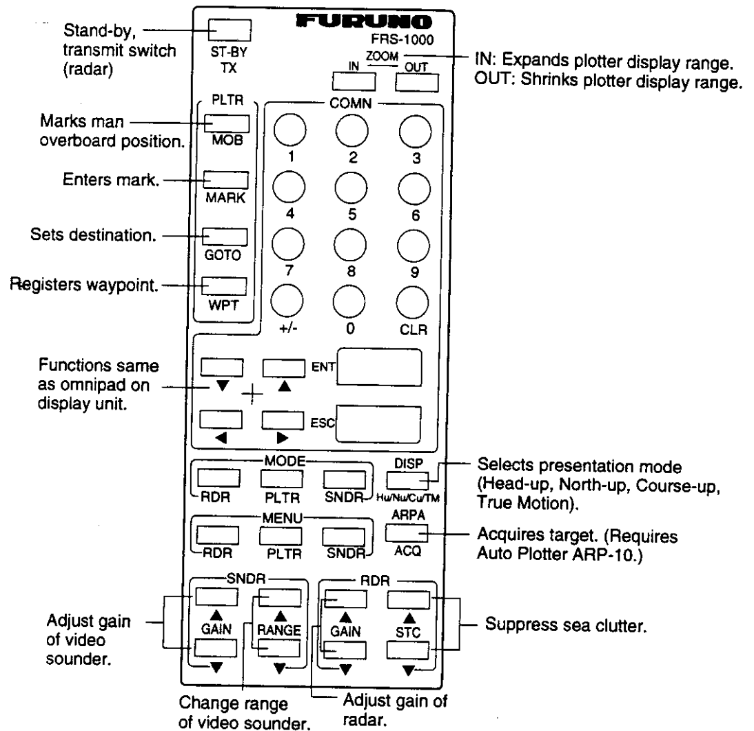
Figure 1-2 Remote controller
