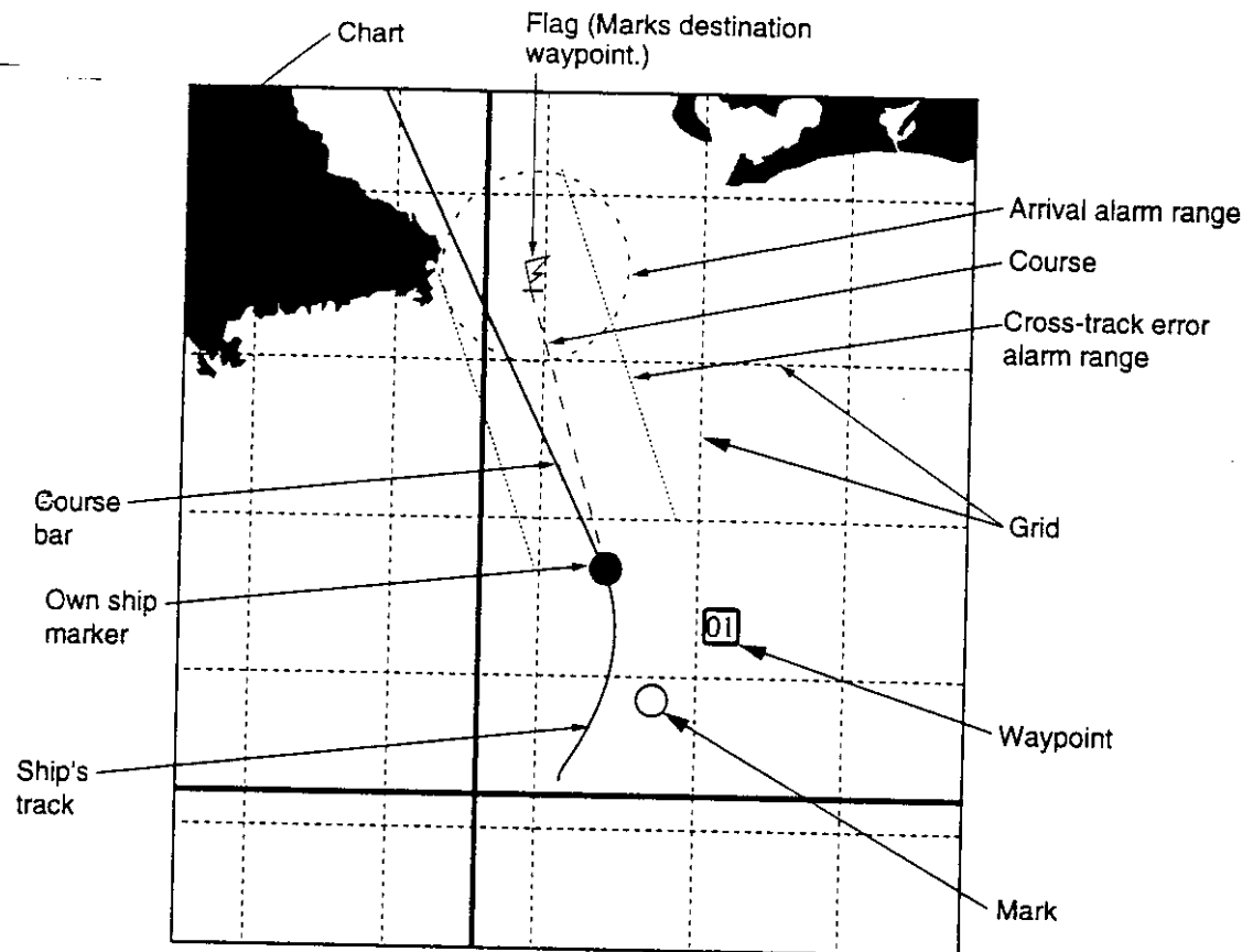
Figure 1-10 Plotter display
