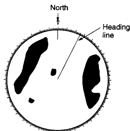
Figure 2-8 North-up presentation mode
