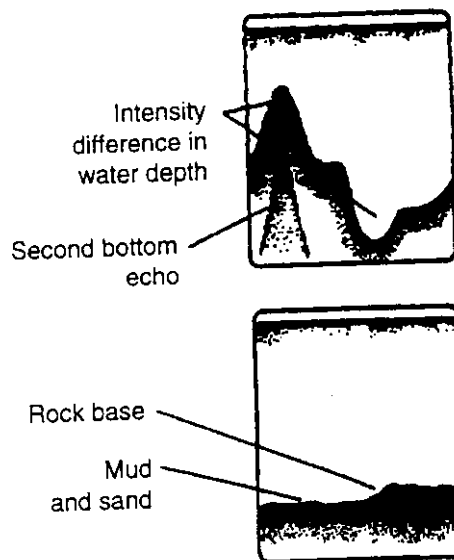
Figure 4-22 Bottom echoes
