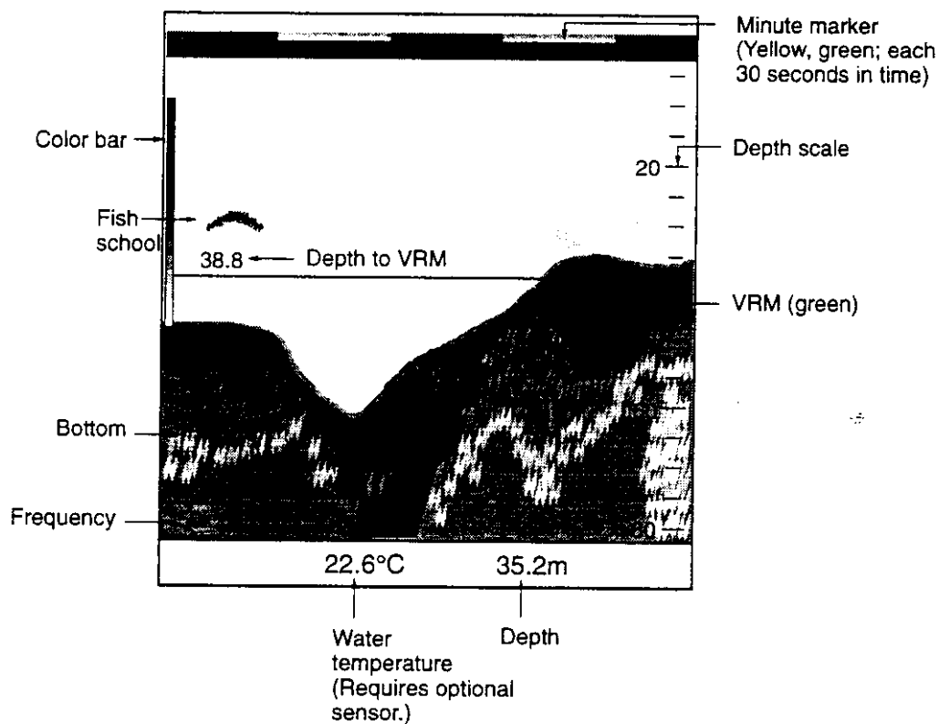
Figure 1-12 Sounder display
