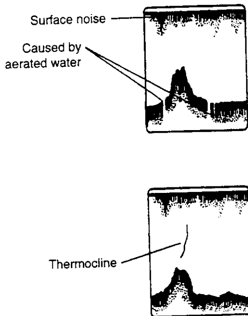
Figure 4-23 Surface noise/aeration
