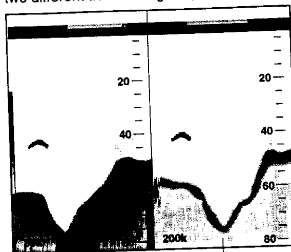
Figure 4-6 Dual-frequency display
