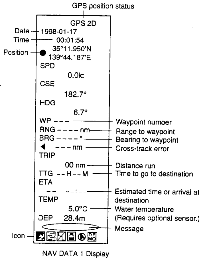
Figure 1-13 Nav data displays
