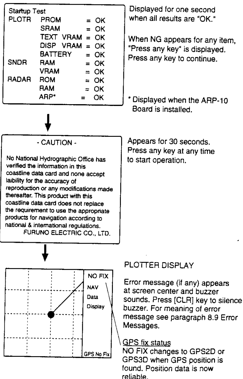
Figure 1-7 Start-up sequence
