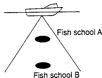
Figure 4-19 TVG concept
