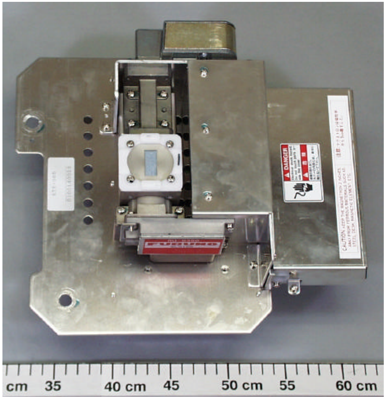
Photo 2.4 Transceiver Module Top View (Showing MIC, Circulator and Magnetron)
