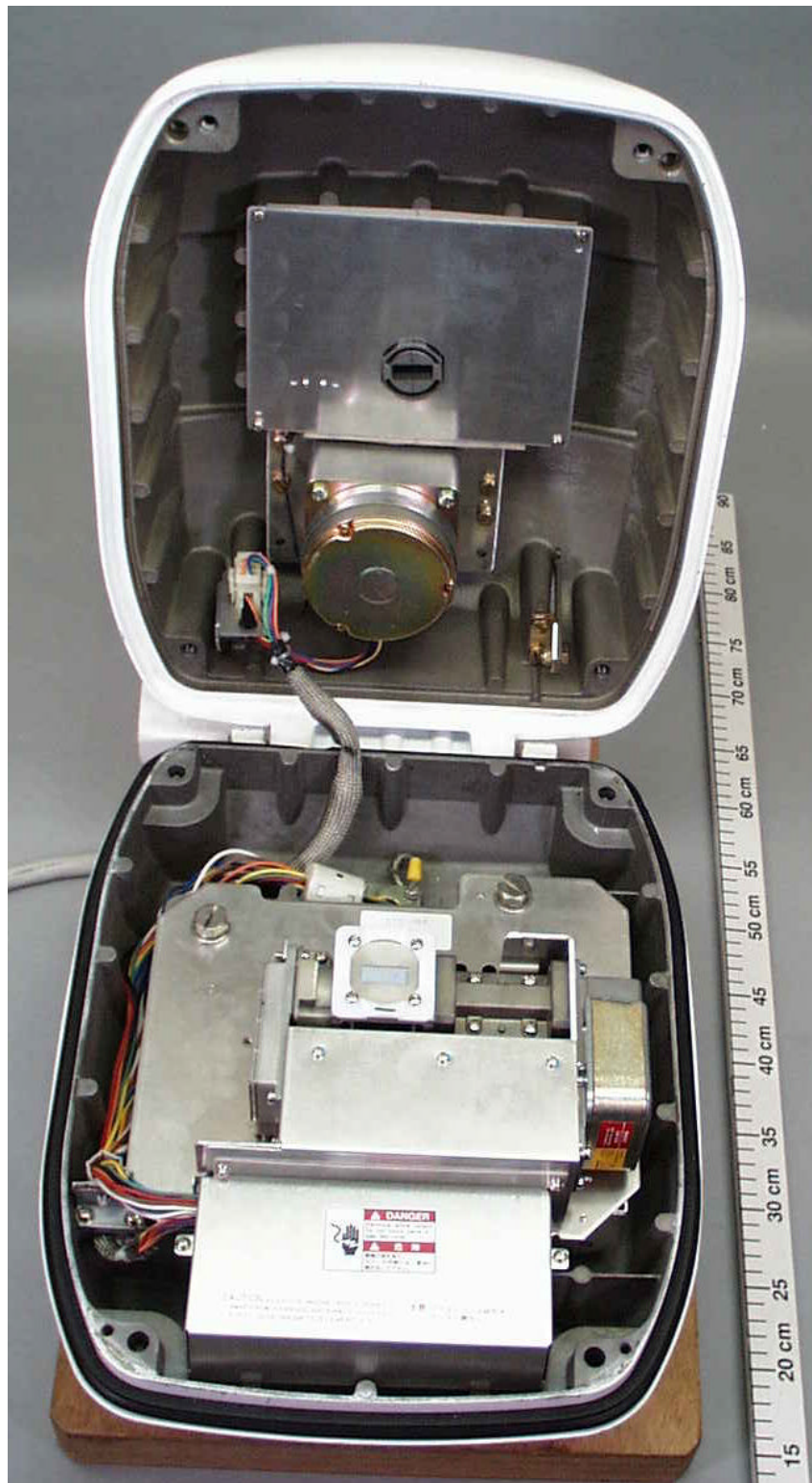
Photo 2.3 Radar Antenna Unit Inside View (Showing Scanner Motor and Transceiver Module)
