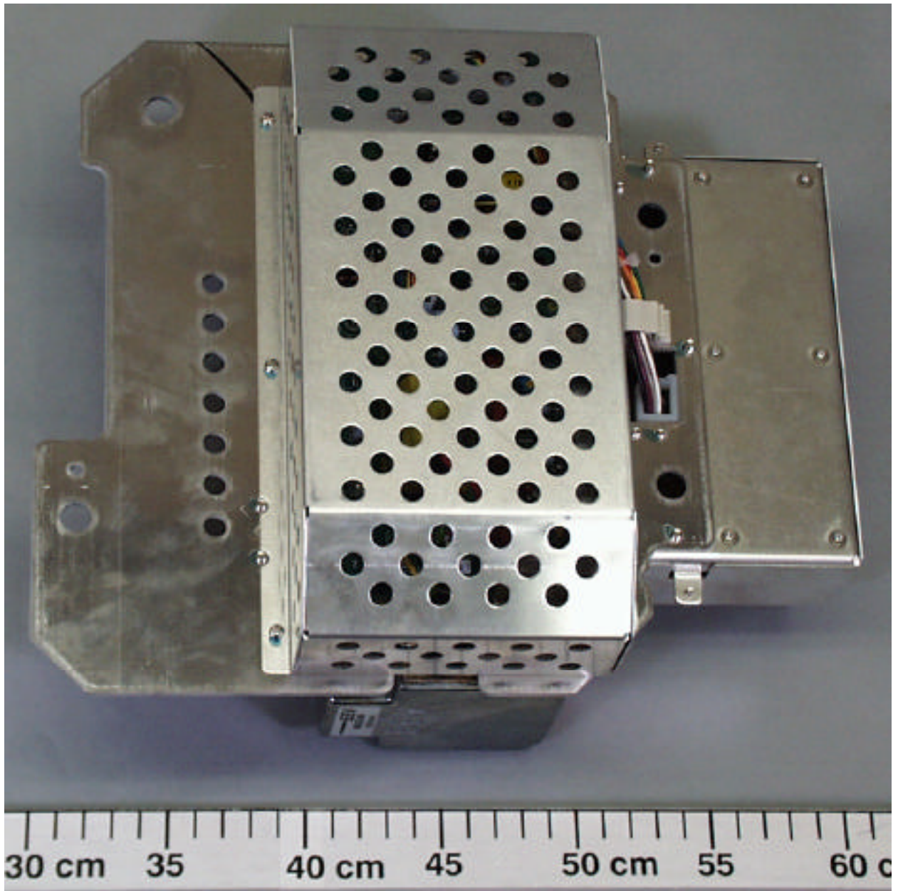
Fig. 2.5 Transceiver Module Bottom View
