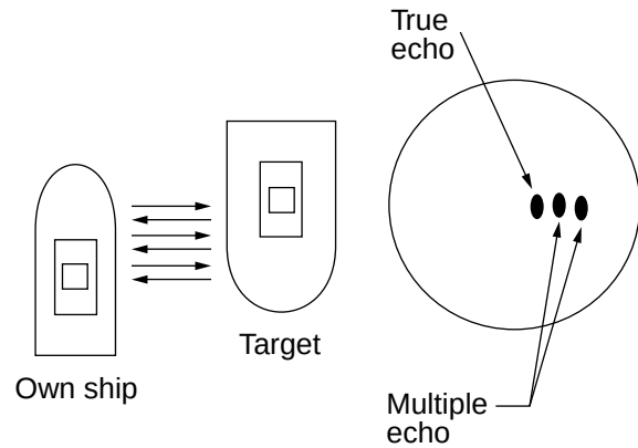
Figure 3-4 Multiple echoes
