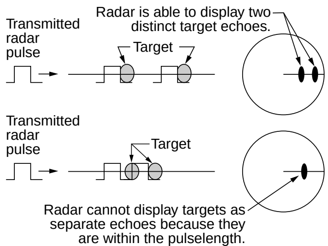
Figure 3-2 Range resolution
