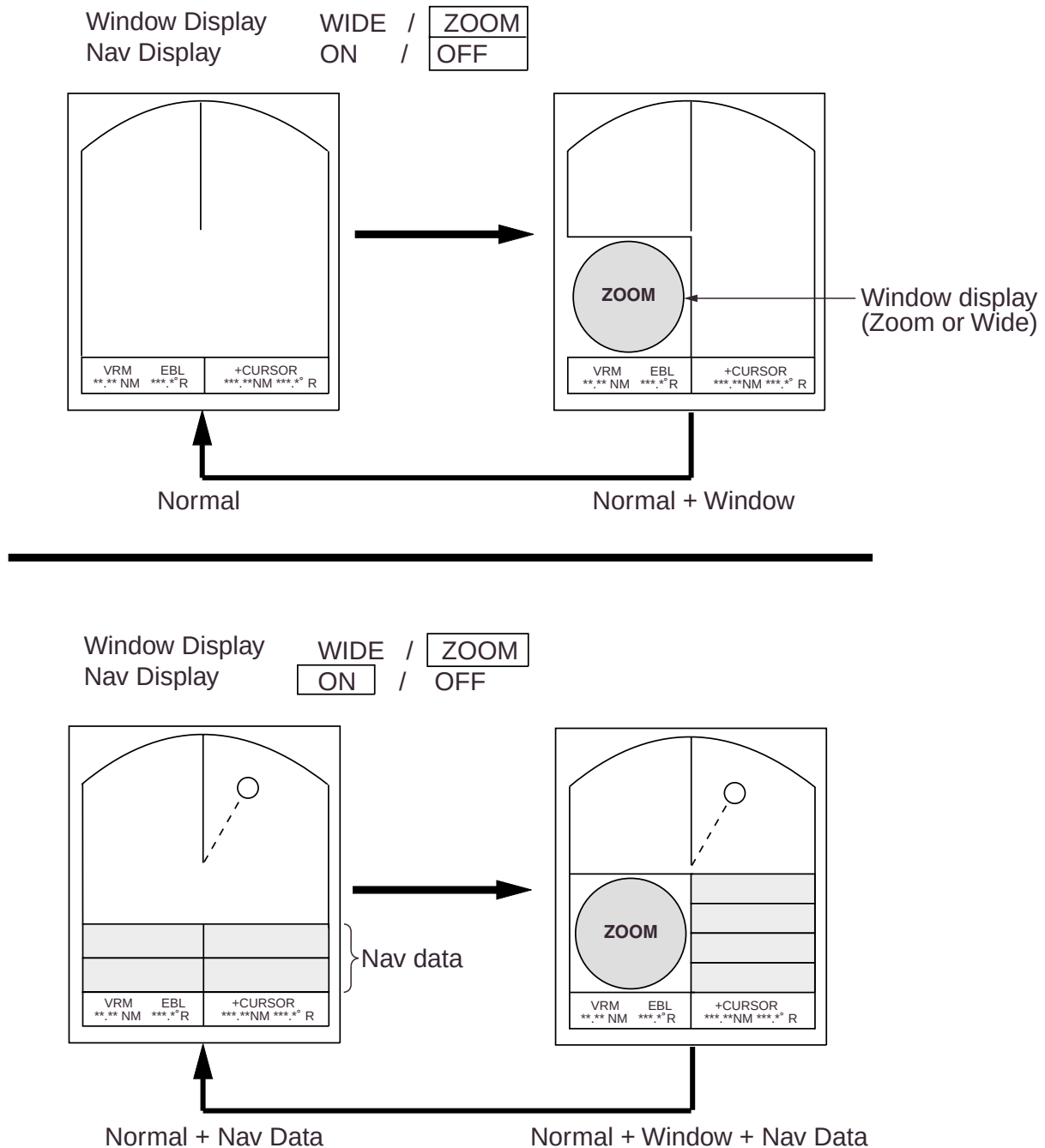
Figure 2-11 Display modes
