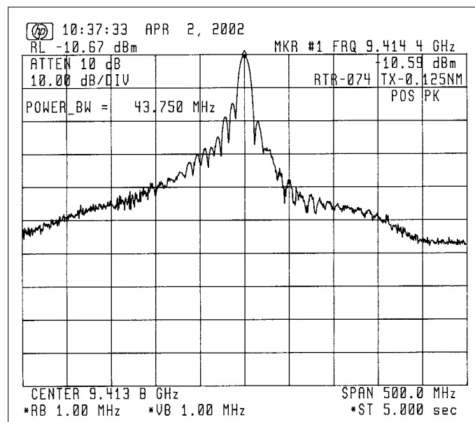
Fig. 3.3.2 Measurement of Occupied Bandwidth
