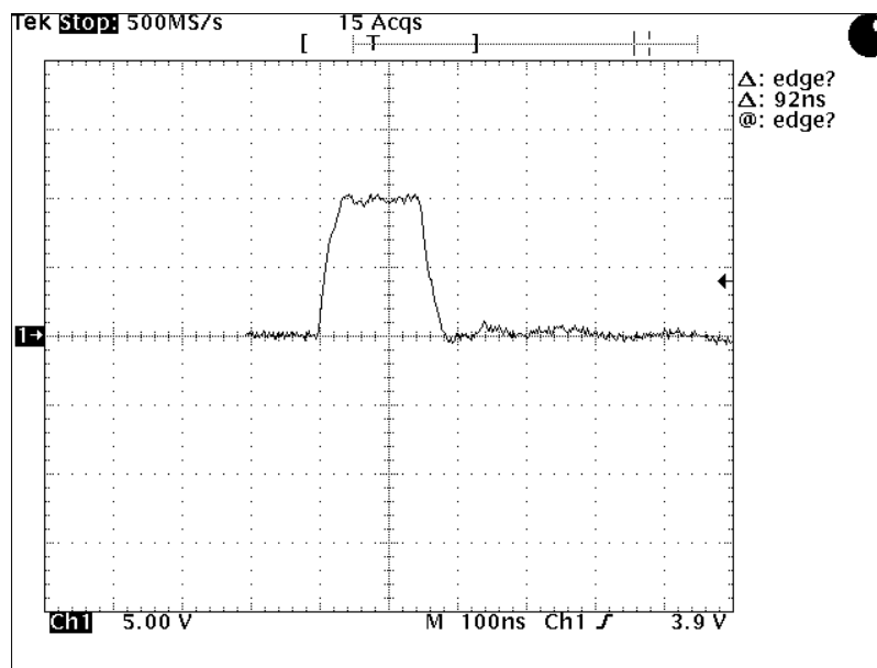
Fig. 3.2.1.1 Typical waveform of Trigger Pulse Scale: 5 V/div., 100 ns/div.
