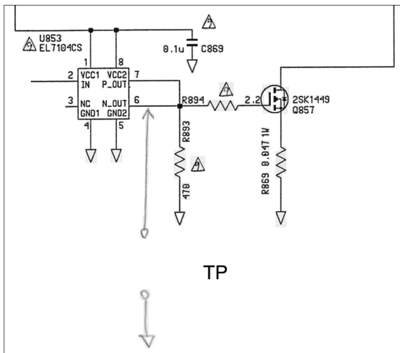
Fig. 3.2.1.2 Test Point for Trigger Pulse (in MD Board (03P9270) of Radar Antenna Unit)
