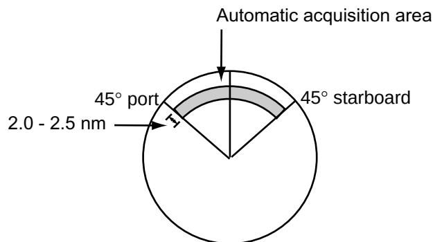
Automatic acquisition area
