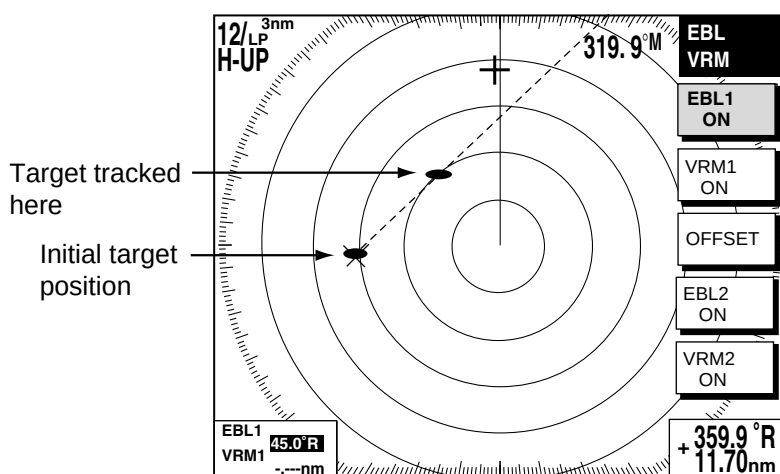
Predicting collision course with the offset EBL
