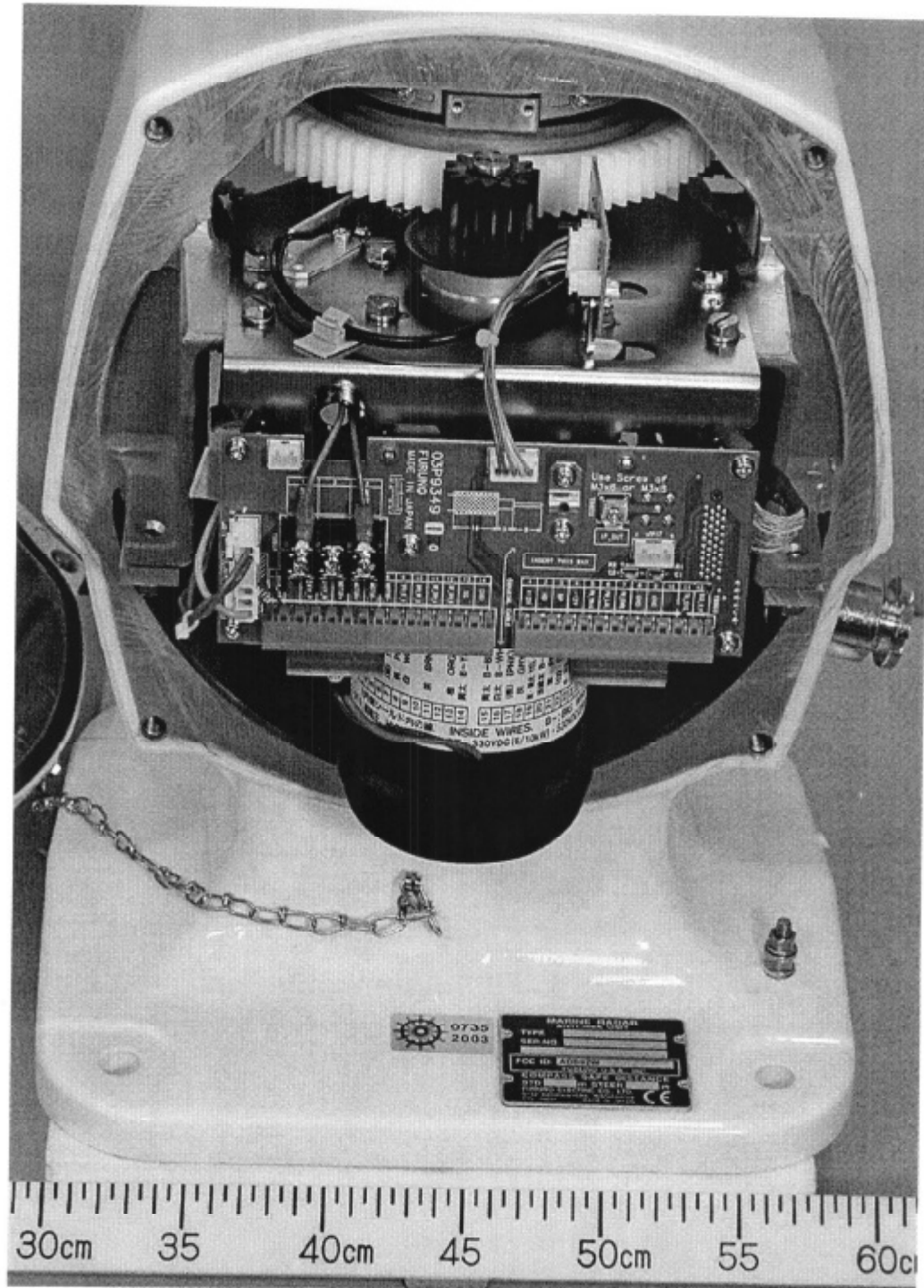
1.3 Inside Front View (with Scanner cover removed, Showing Scanner Motor and TB Board 03P9349)
