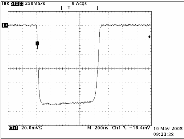
Fig. 3.2.3.5 Long 2 Pulse (48 nm Range) Scale: 20 mV/div. 200 ns/div.
