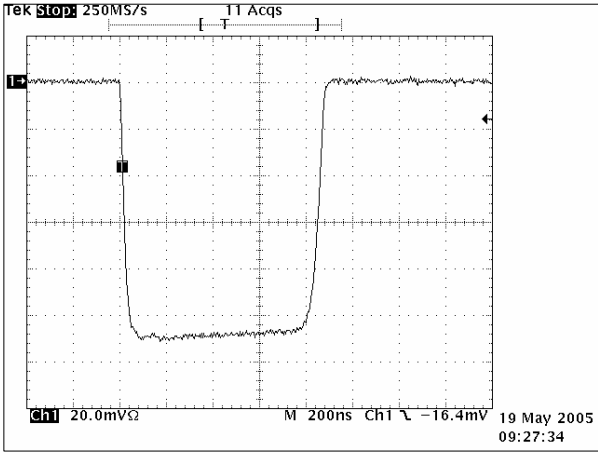
Fig. 3.2.3.6 Long 3 Pulse (72 nm Range) Scale: 20 mV/div. 200 ns/div.
