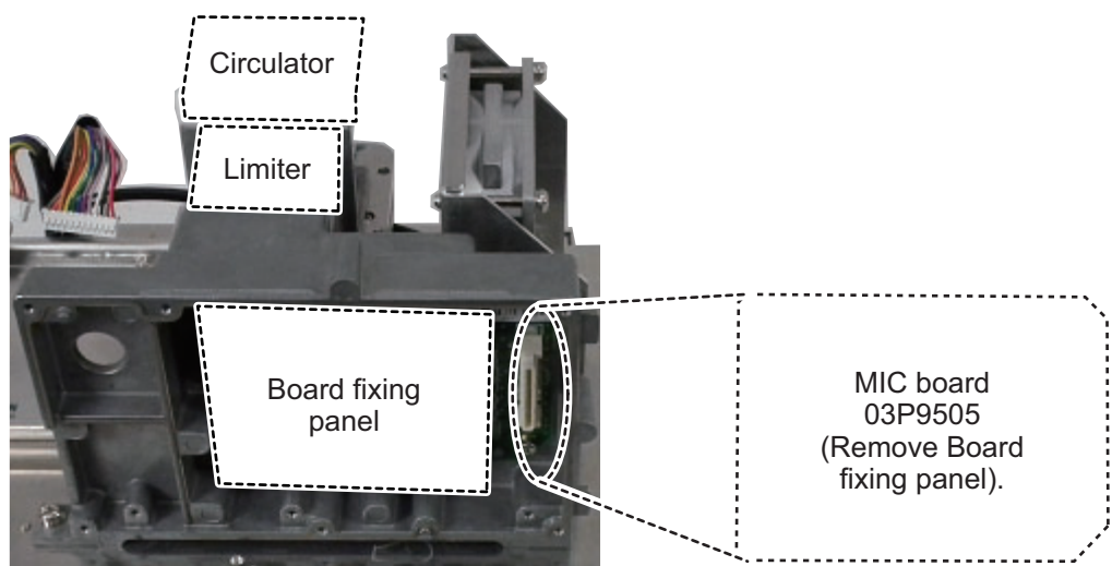
Transceiver module RTR-101 underside-front view (For FAR-1518/1528/BB)
