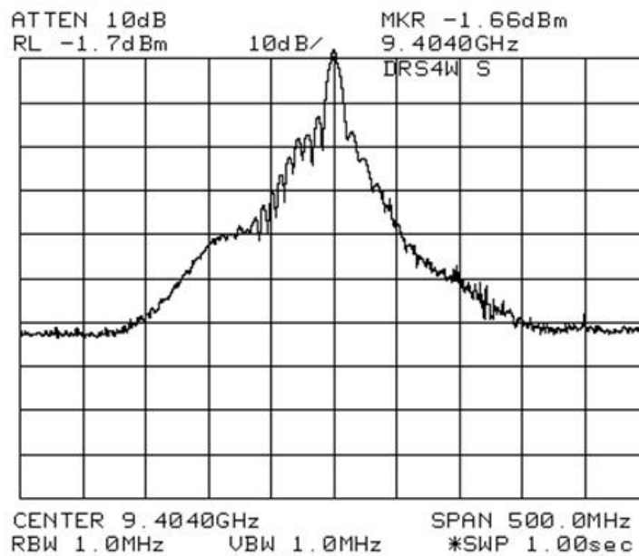
Fig. 7.1 S Pulse Envelope and Spectrum
