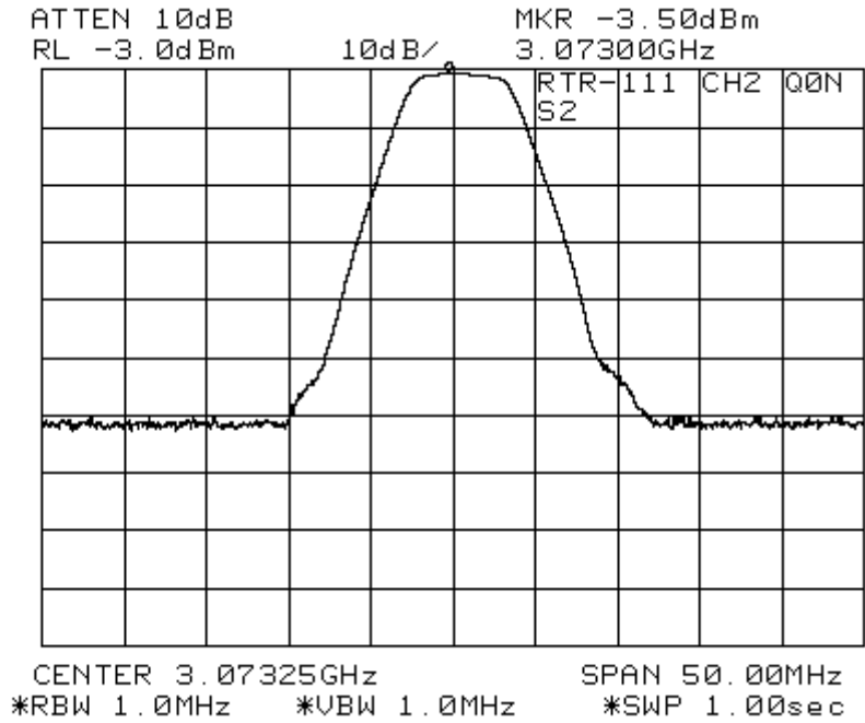
Fig. 7.23 S2 Pulse Envelope and Spectrum
