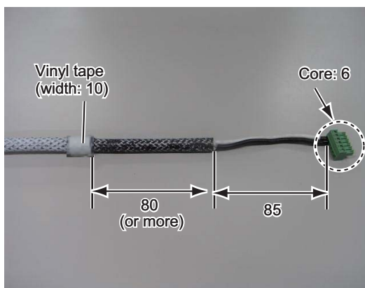
DPYC-1.5 cable
