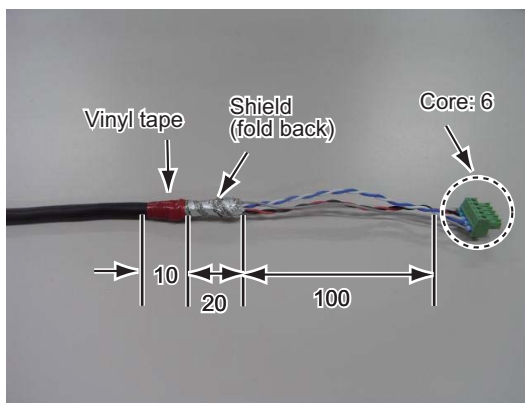
MC1.5-W-L600/1000/2000/3000 cable
