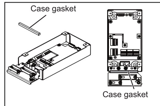
Chassis
