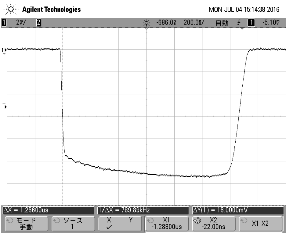
Fig. 7.6 L Pulse Envelope
