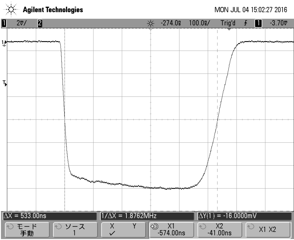
Fig. 7.4 M2 Pulse Envelope
