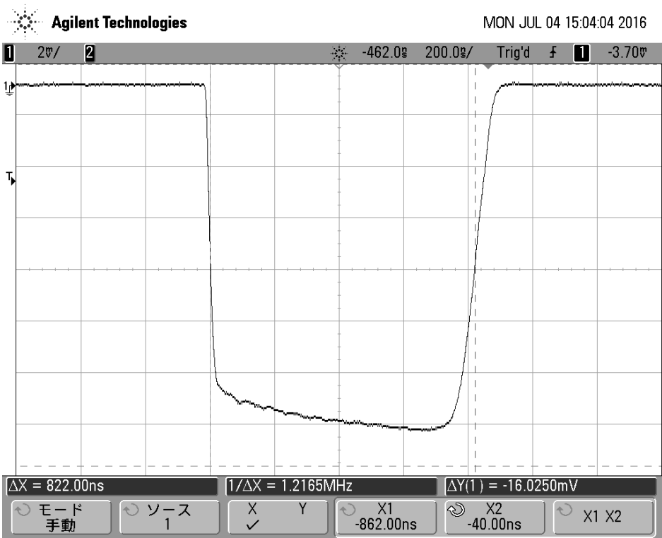
Fig. 7.5 M3 Pulse Envelope
