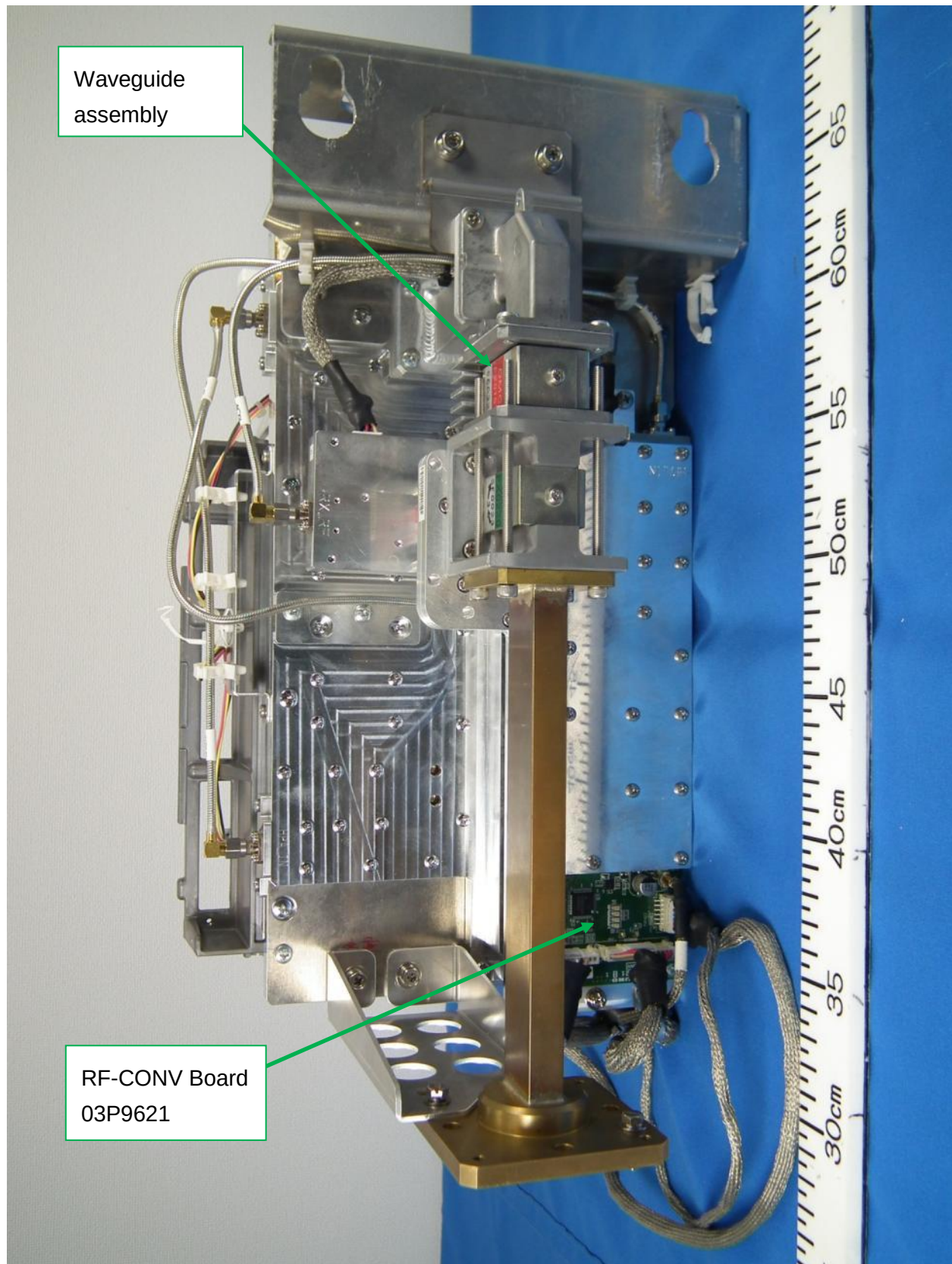
2.8 RF unit rear side view
