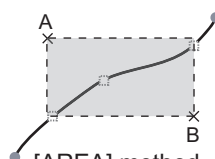
[AREA] method
