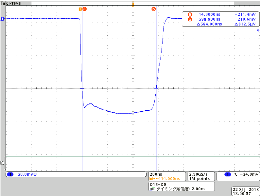
Fig. 6.4 L pulse envelope
