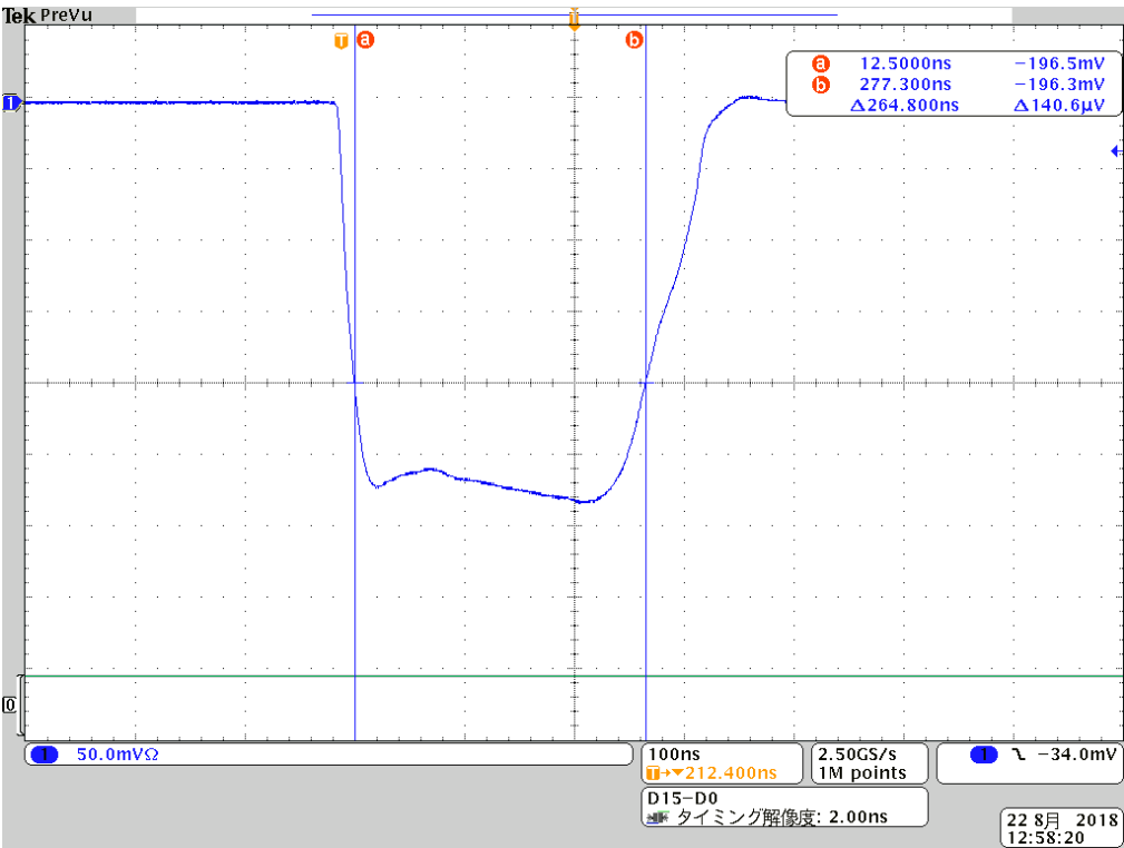
Fig. 6.3 M2 pulse envelope
