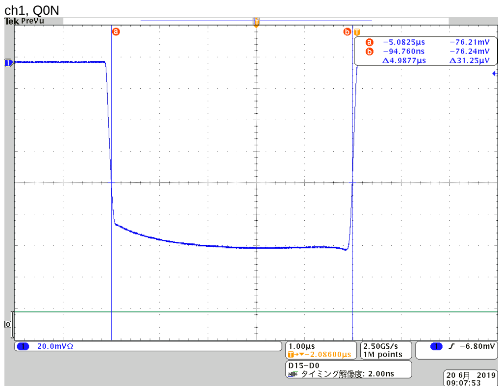
Fig. 6.10 ch1, Q0N, S0 pulse envelope
