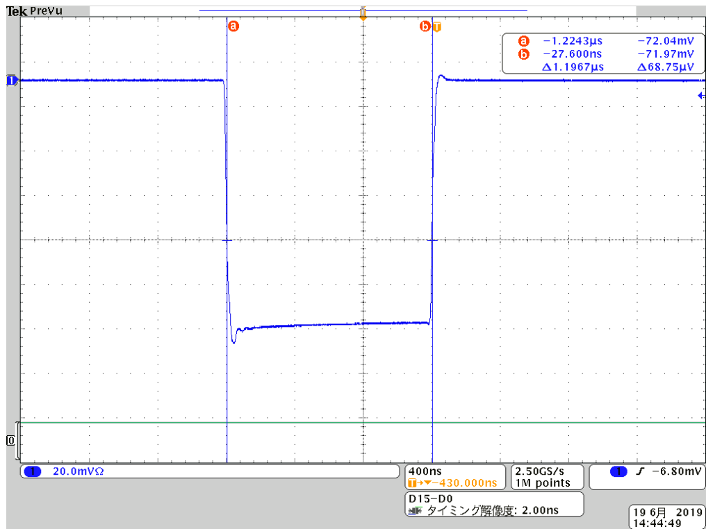
Fig. 6.9 ch1, P0N, L2 pulse envelope
