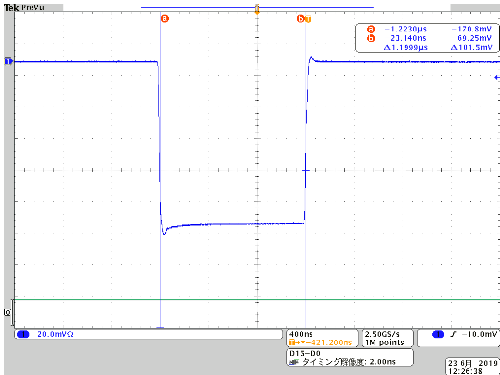
Fig. 6.25 ch2, P0N, L1 pulse envelope
