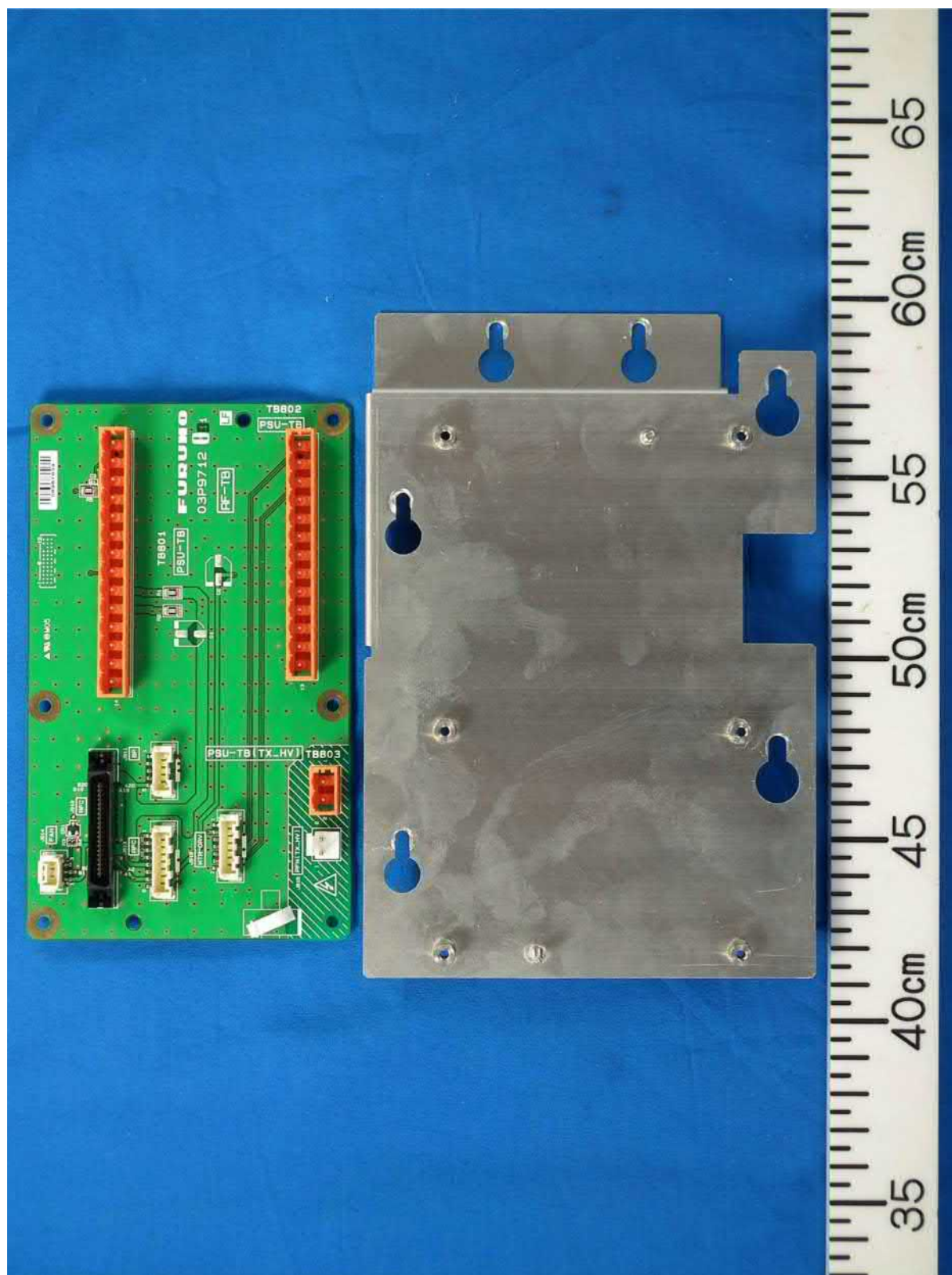
1.5 RF-TB board module (with removed from the metal base part)
