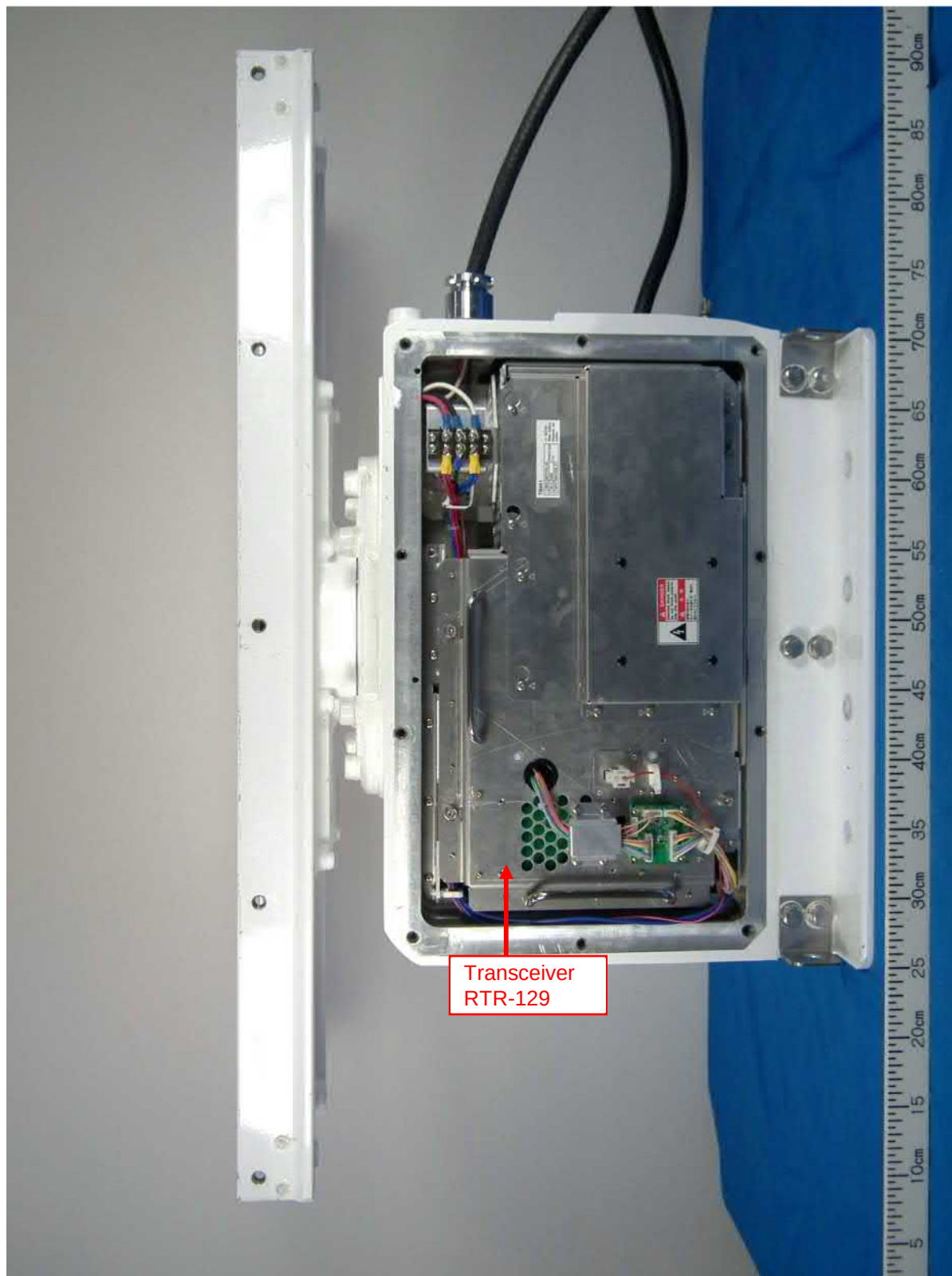
1.16 Left side view (with the left side cover removed, showing Transceiver RTR-129)
