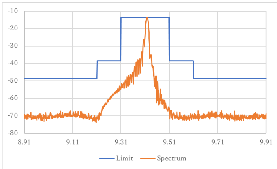
Fig. 7.7 S1 pulse
