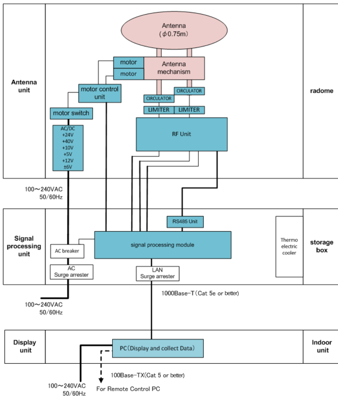
Block diagram
