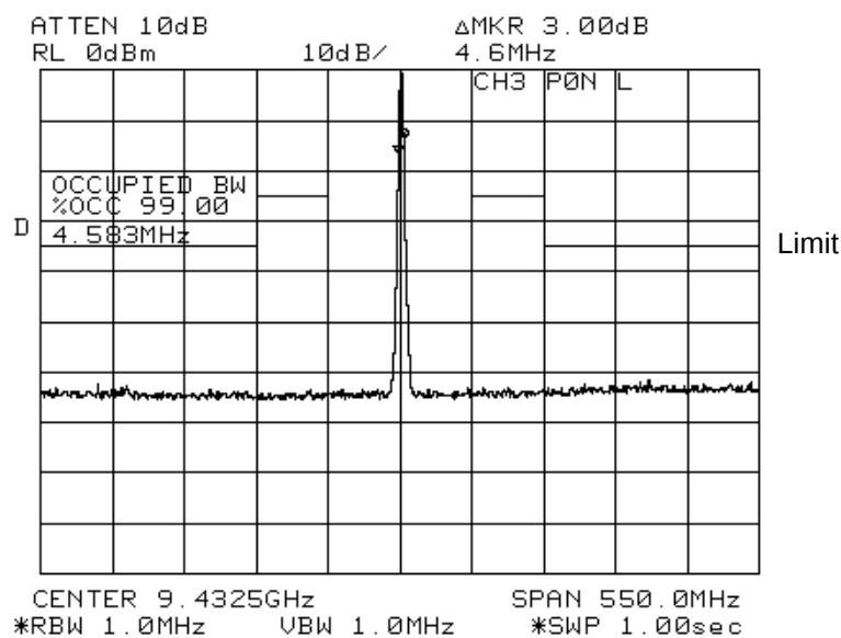
Fig. 7.10 CH3, Horizontal, P0N, Long pulse
