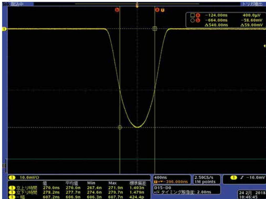
Fig. 6.13 Short pulse envelope
