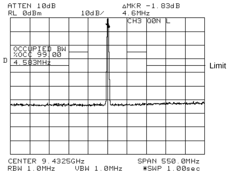
Fig. 7.16 CH3, Vertical, Q0N, Long pulse
