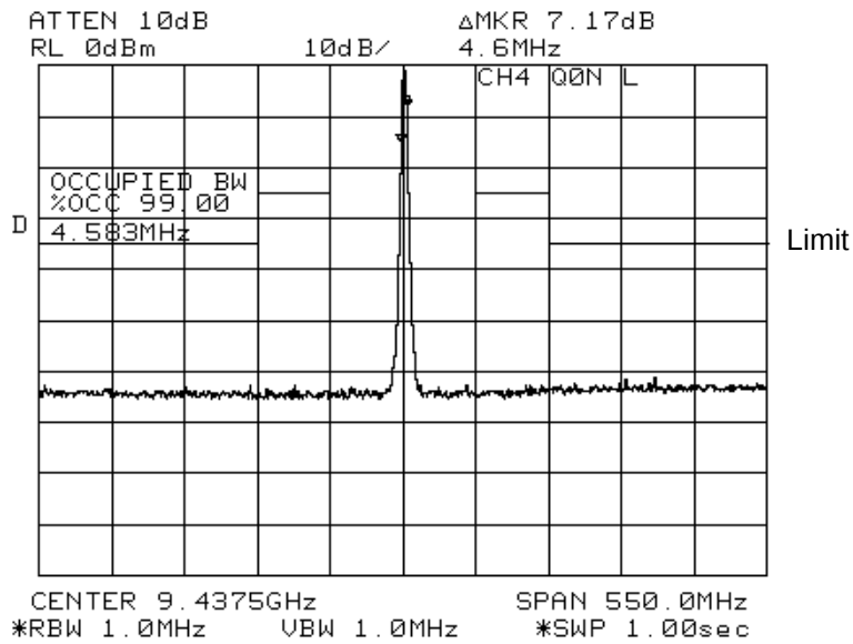
Fig. 7.20 CH4, Horizontal, Q0N, Long pulse
