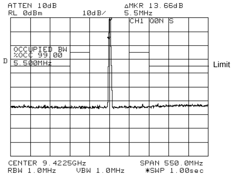
Fig. 7.7 CH1, Vertical, Q0N, Short pulse
