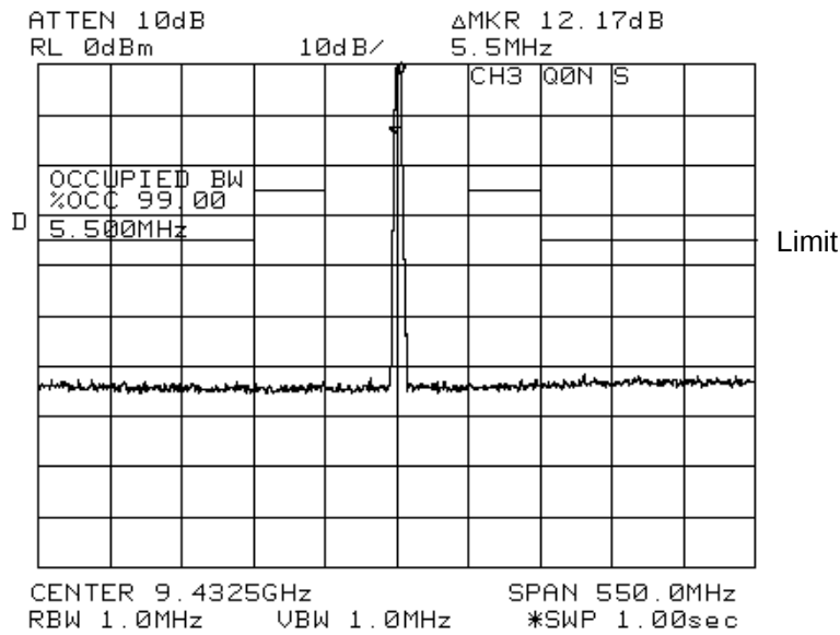
Fig. 7.15 CH3, Vertical, Q0N, Short pulse
