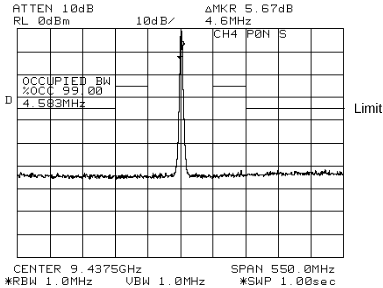
Fig. 7.17 CH4, Horizontal, P0N, Short pulse
