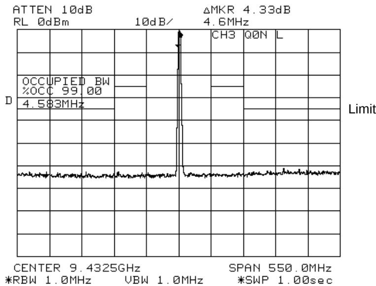
Fig. 7.12 CH3, Horizontal, Q0N, Long pulse
