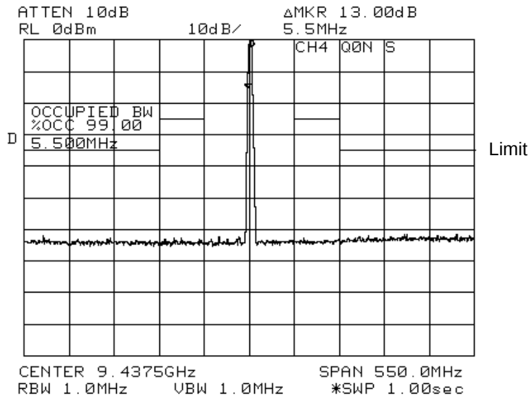
Fig. 7.23 CH4, Vertical, Q0N, Short pulse
