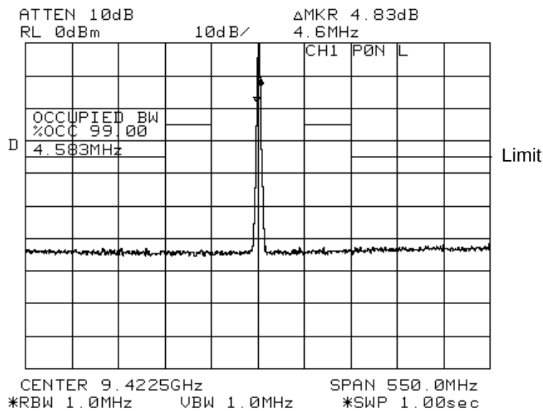
Fig. 7.2 CH1, Horizontal, P0N, Long pulse
