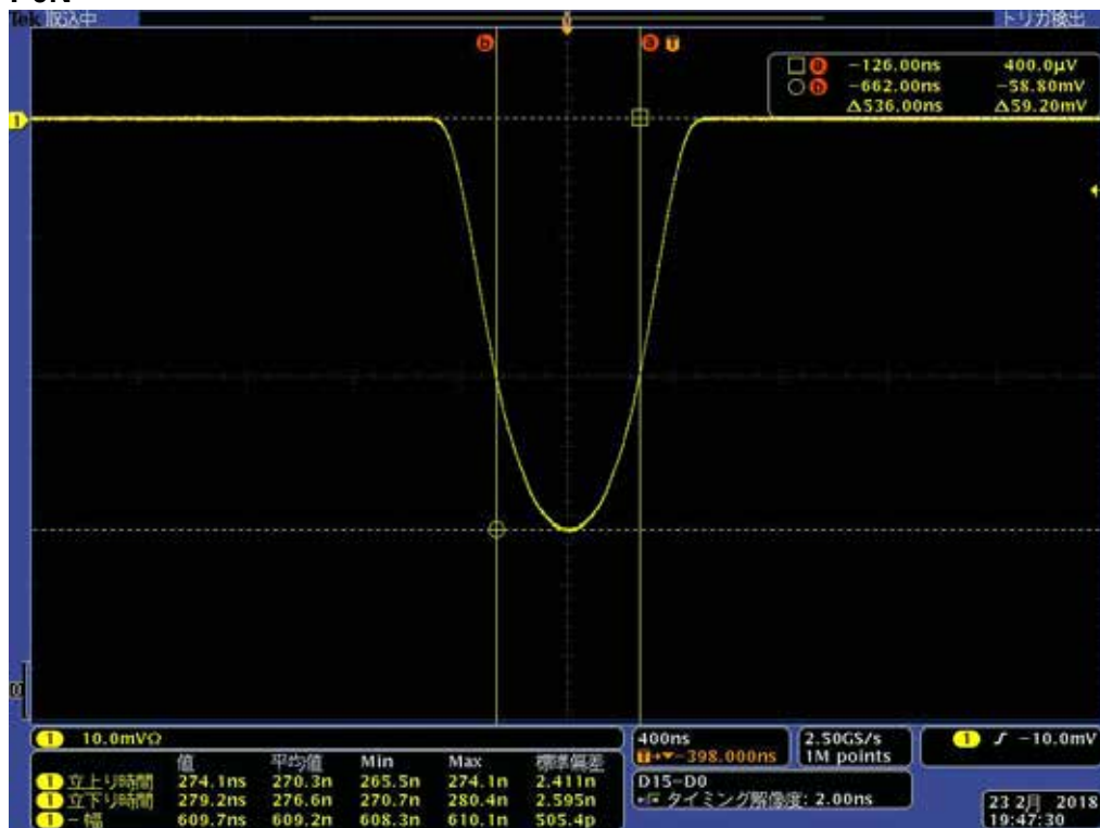
Fig. 6.17 Short pulse envelope
