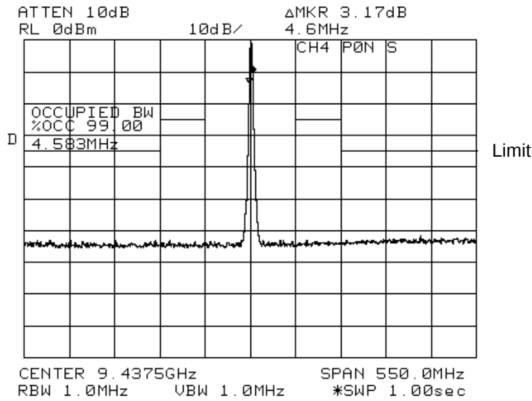
Fig. 7.21 CH4, Vertical, P0N, Short pulse
