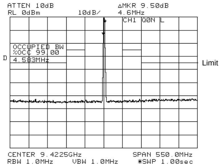
Fig. 7.8 CH1, Vertical, Q0N, Long pulse
