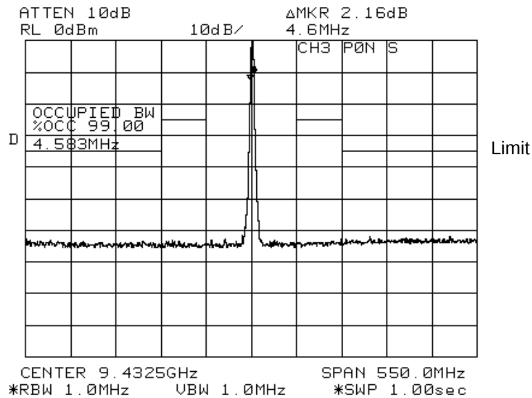
Fig. 7.9 CH3, Horizontal, P0N, Short pulse
