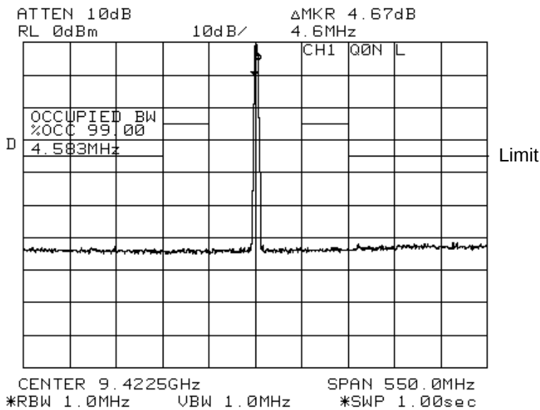
Fig. 7.4 CH1, Horizontal, Q0N, Long pulse
