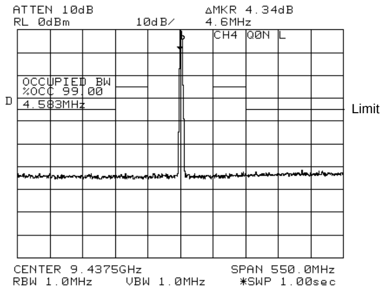
Fig. 7.24 CH4, Vertical, Q0N, Long pulse
