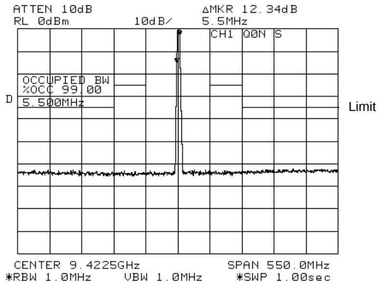
Fig. 7.3 CH1, Horizontal, Q0N, Short pulse
