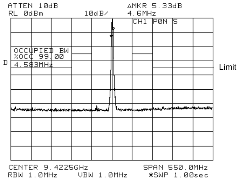
Fig. 7.5 CH1, Vertical, P0N, Short pulse
