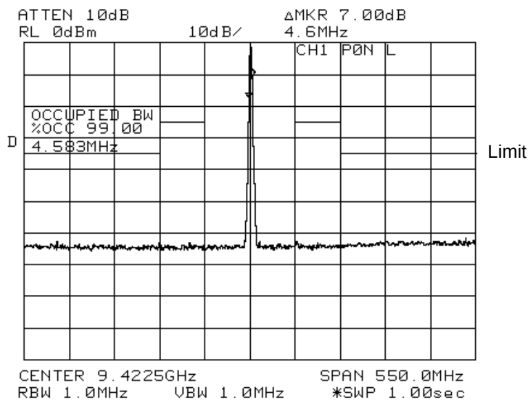
Fig. 7.6 CH1, Vertical, P0N, Long pulse
