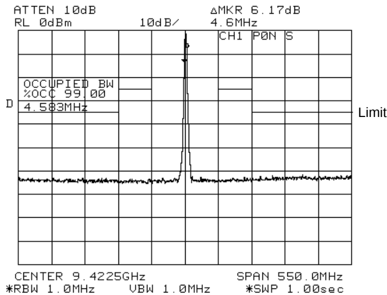
Fig. 7.1 CH1, Horizontal, P0N, Short pulse
