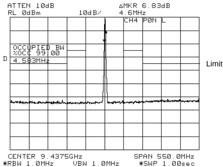
Fig. 7.18 CH4, Horizontal, P0N, Long pulse
