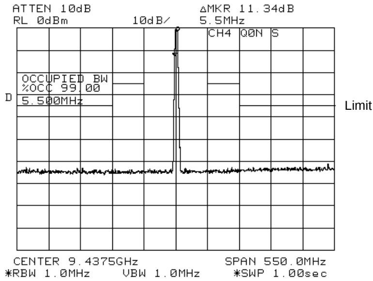
Fig. 7.19 CH4, Horizontal, Q0N, Short pulse
