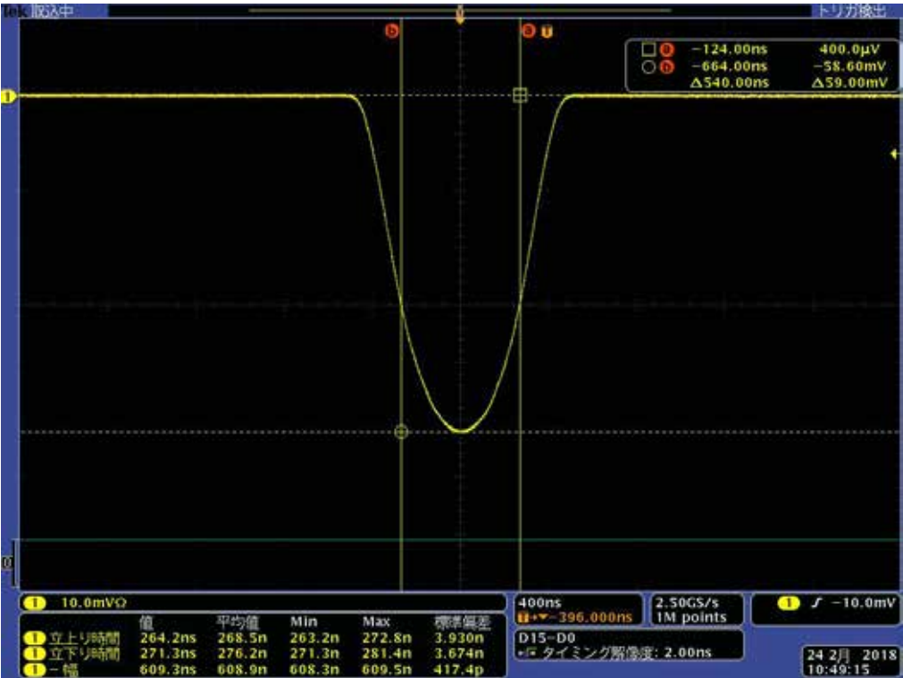
Fig. 6.21 Short pulse envelope
