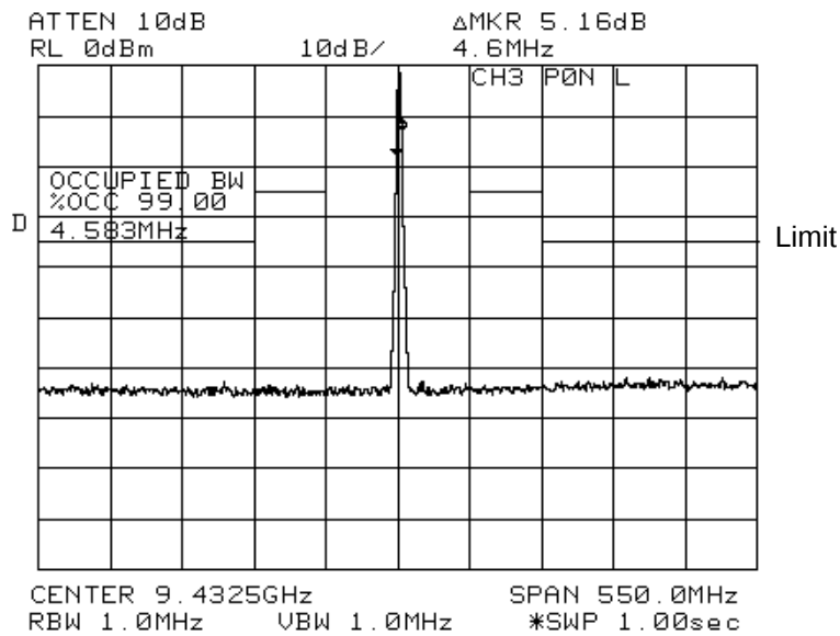
Fig. 7.14 CH3, Vertical, P0N, Long pulse
