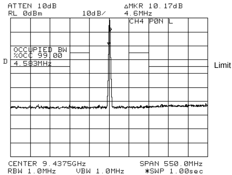
Fig. 7.22 CH4, Vertical, P0N, Long pulse
