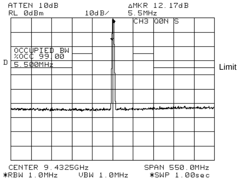
Fig. 7.11 CH3, Horizontal, Q0N, Short pulse
