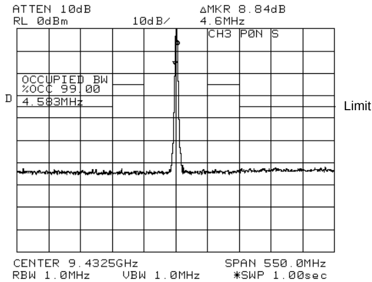
Fig. 7.13 CH3, Vertical, P0N, Short pulse
