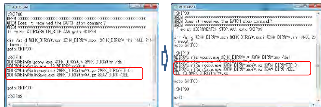
Figure 4.9: Sample of AUTO.bat (Before -&gt; After)
