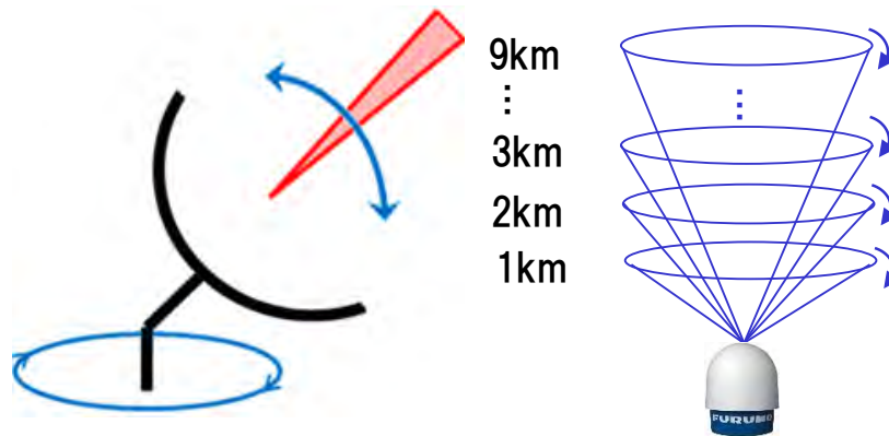
Figure 5.1: Basic volume scan
