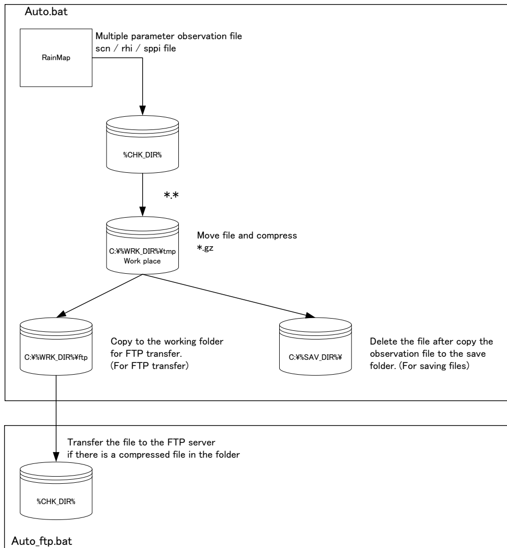
Figure 4.3: WR_transfer.bat processing contents
