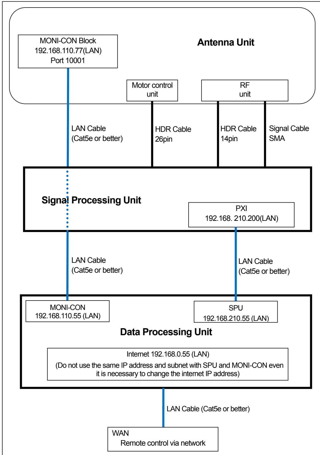
Image 2: Configuration diagram
