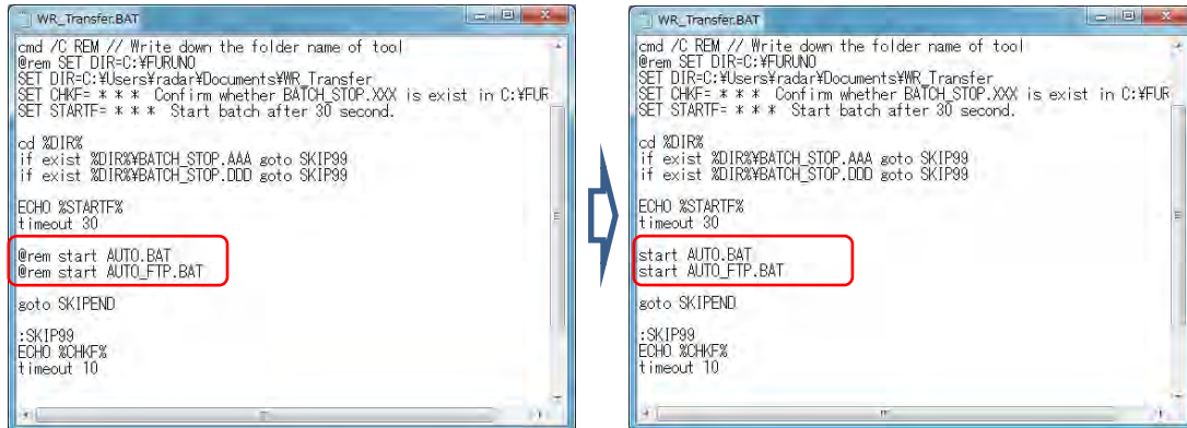
Figure 4.10: Sample of WR_transfer.bat (Before -> After)
