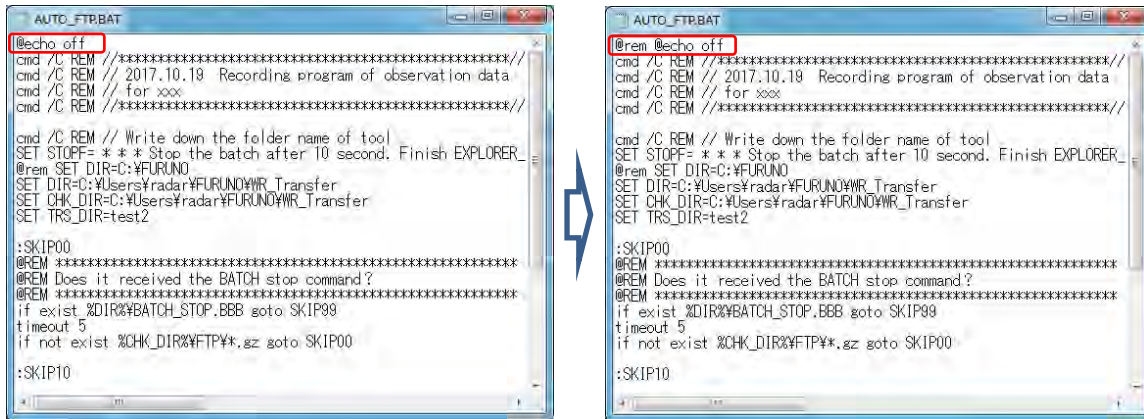
Figure 4.12: Sample of AUTO_FTP.bat (Before -> After)
