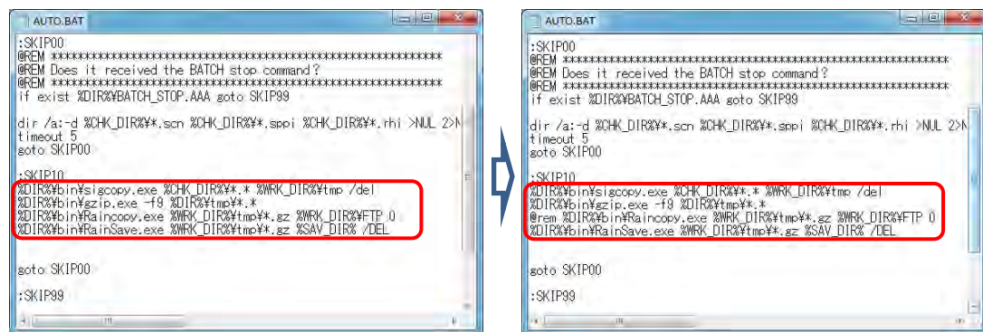
Figure 4.8: Sample of AUTO.bat (Before -&gt; After)
