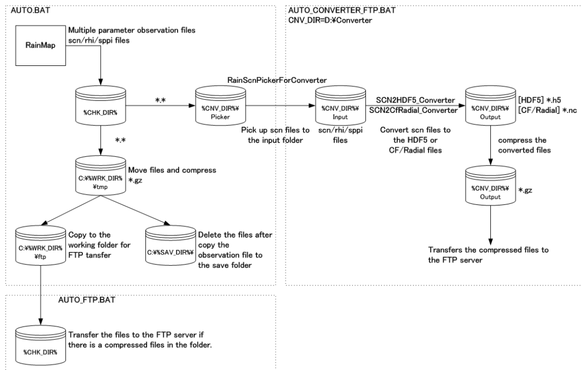
Figure 4.15: Data flow for data converter
