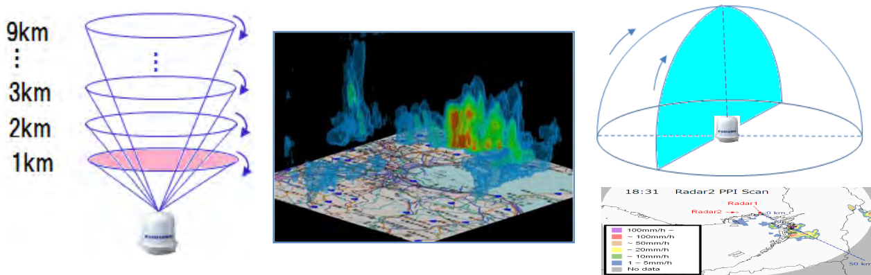
Figure 2.10: Outline of slice mode
