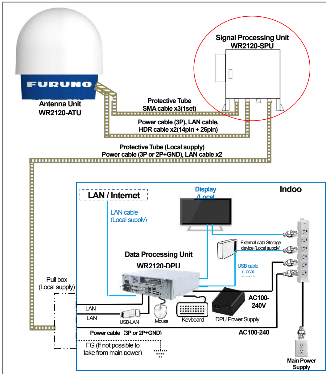
Image 1: System drawing
