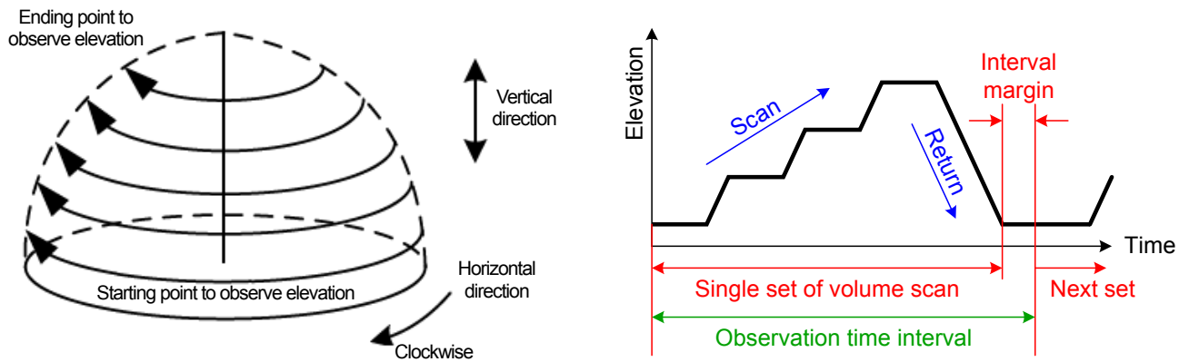
Figure 2.7: Volume scan mode
