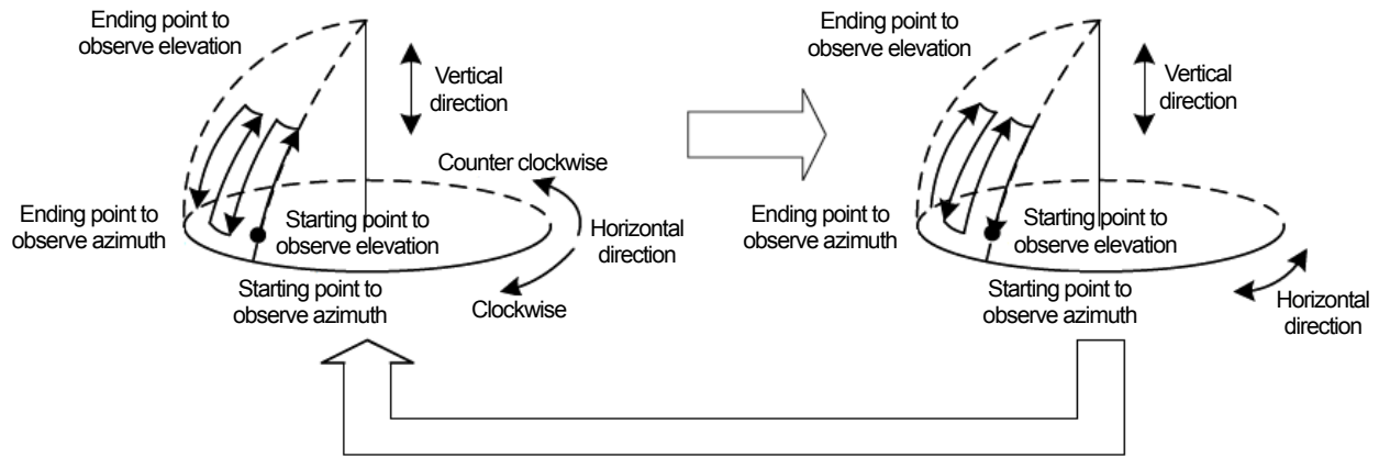
Figure 2.6: SRHI scan mode
