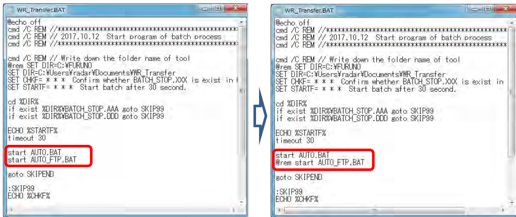
Figure 4.7: Sample of WR_transfer.bat (Before -&gt; After)
