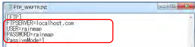
Figure 4.6: Sample of FTP_WR_FTP.ini
