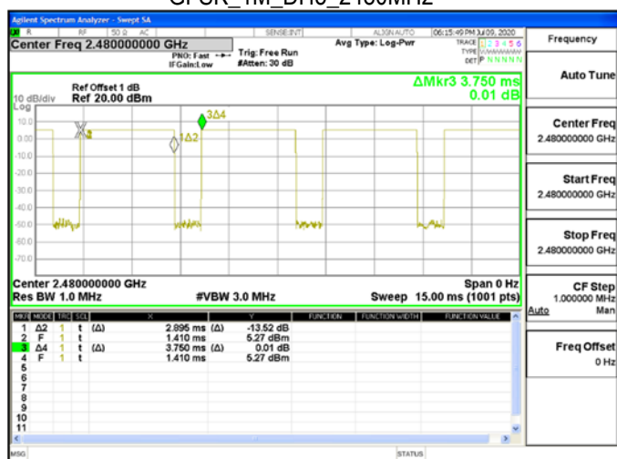
GFSK_1M_DH5_2480MHz
