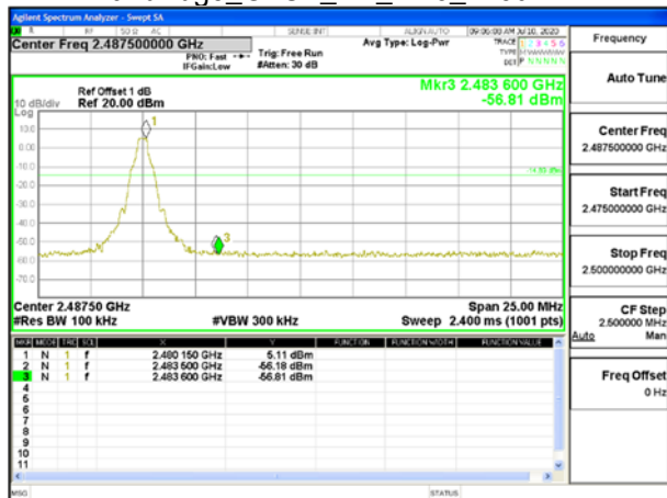
BandEdge_GFSK_1M_DH5_2480MHz
