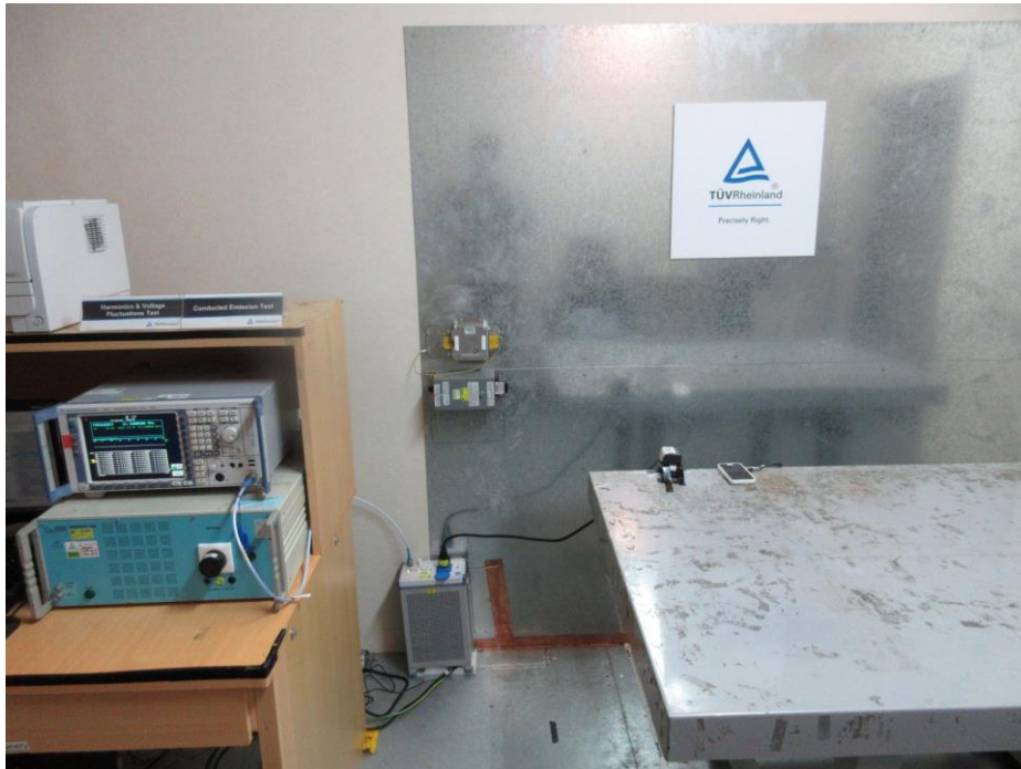
Photograph 7: Set-up for Mains Conducted testing (Front View)
