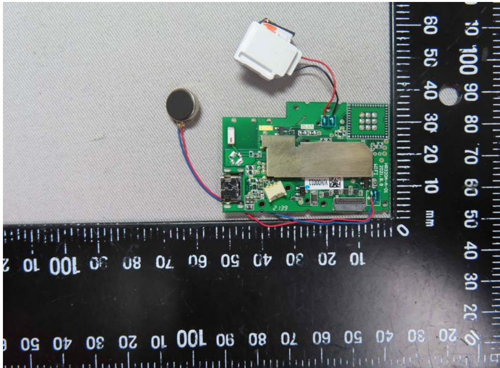
Internal View of EUT – 1 (Panel A)
