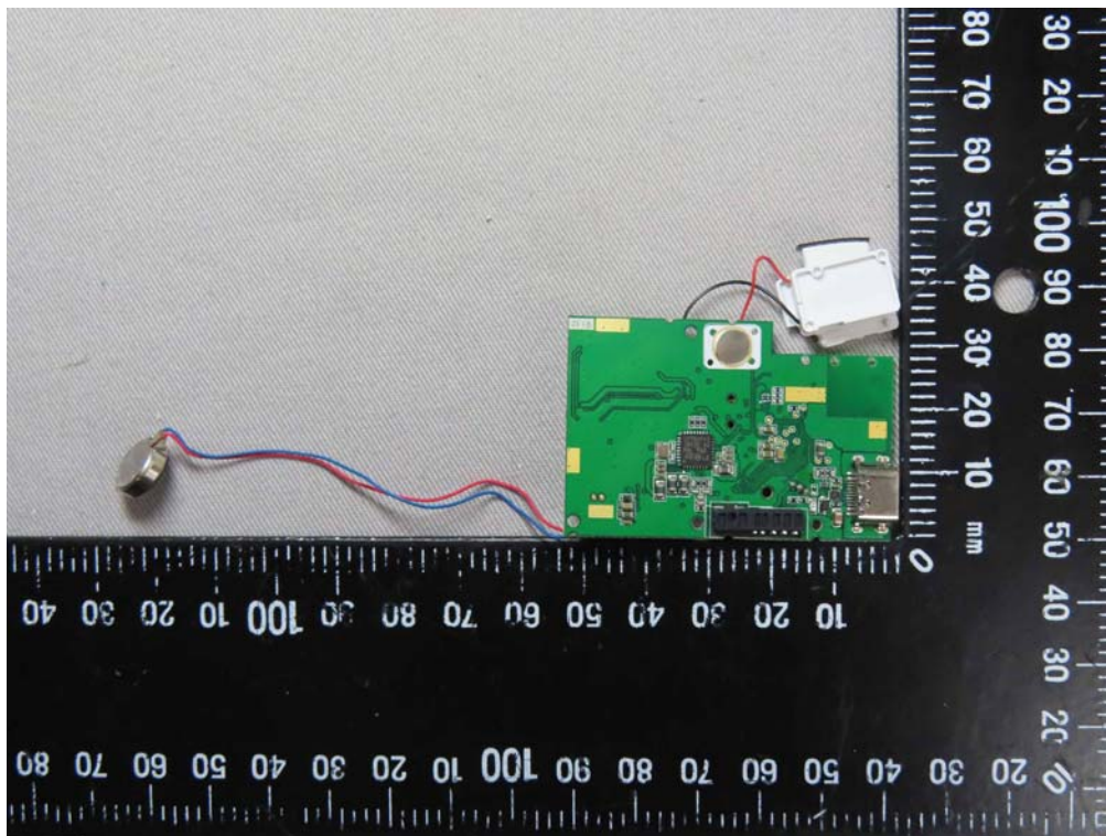
Internal View of EUT – 1 (Panel B)
