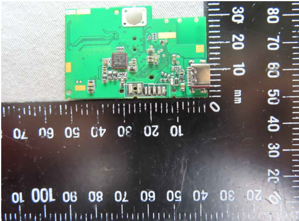
Internal View of EUT – 1 (Panel B)
