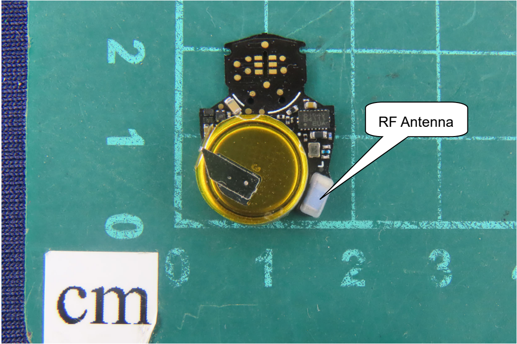
(79) EUT Photo
