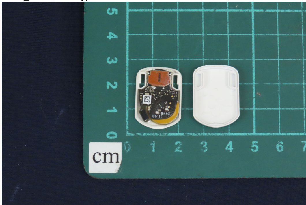
(80) EUT Photo_M/N: HT513 Type D
