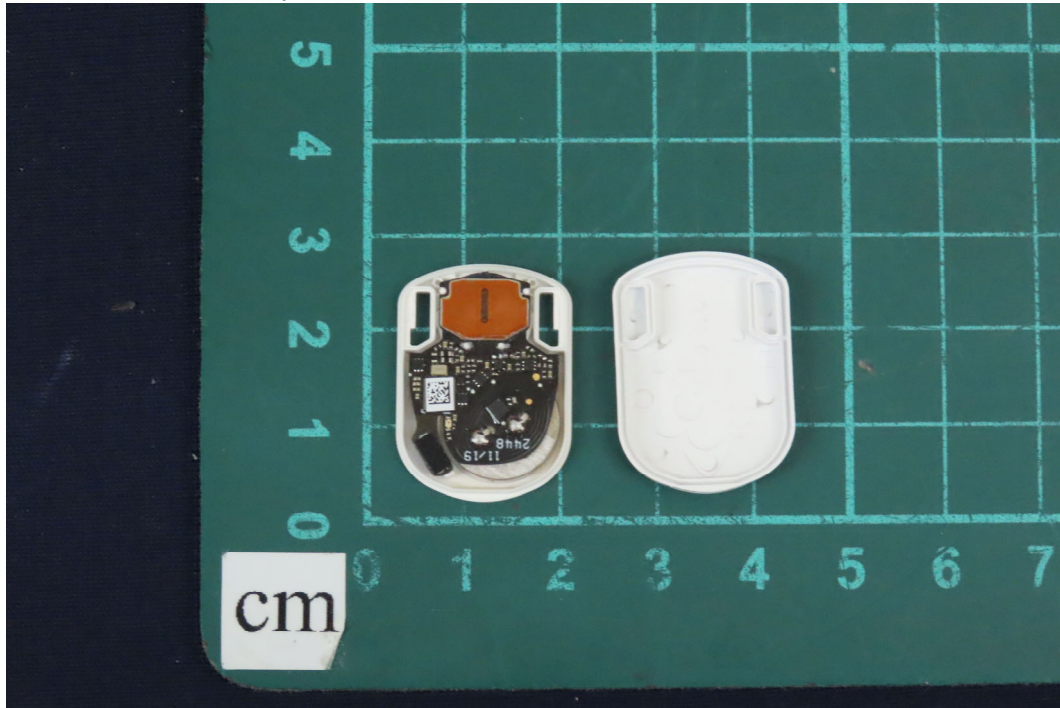
(52) EUT Photo_M/N: HT510 Type A
