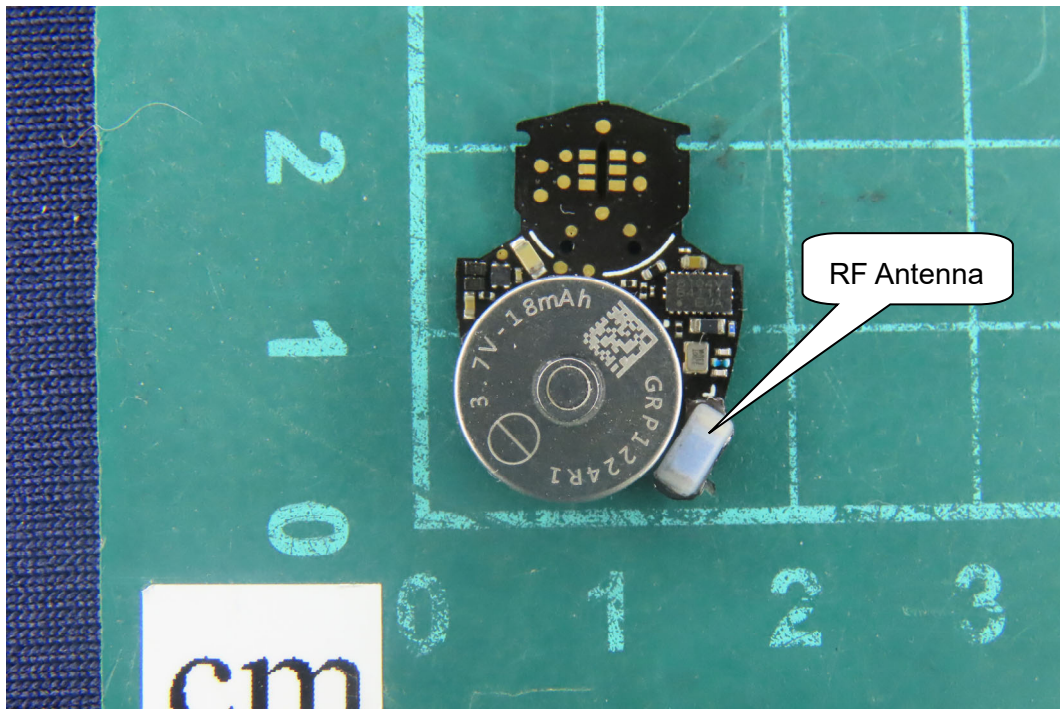
(55) EUT Photo
