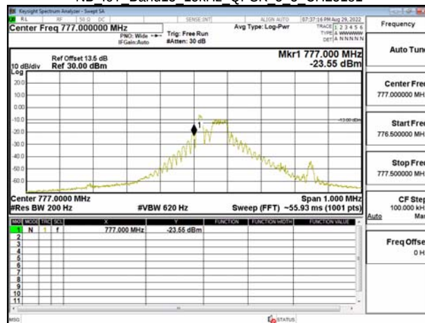
NB IoT Band13 15kHz QPSK 3 3 CH23279
