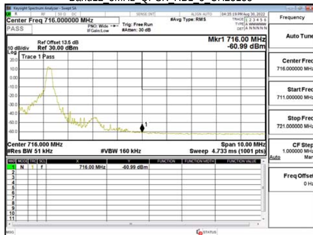
Band12 5MHz QPSK RB1 5 CH23155
