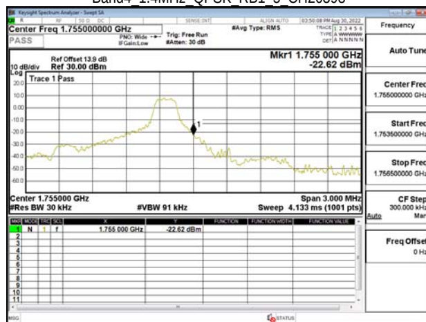
Band4 1.4MHz QPSK RB1 5 CH20393
