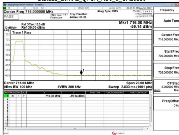
Band12 10MHz QPSK RB6 0 CH23130
