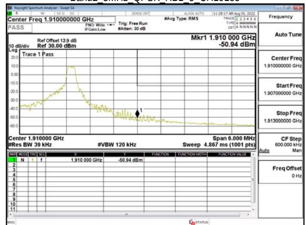
Band2 3MHz QPSK RB1 5 CH19185
