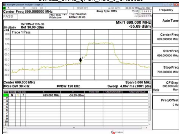
Band12 3MHz QPSK RB6 0 CH23025
