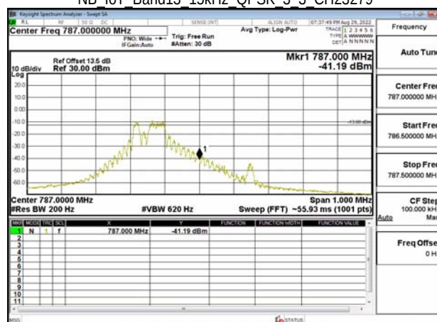
NB IoT Band13 15kHz QPSK 3 3 CH23279
