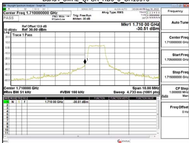
Band4 5MHz QPSK RB6 0 CH19975
