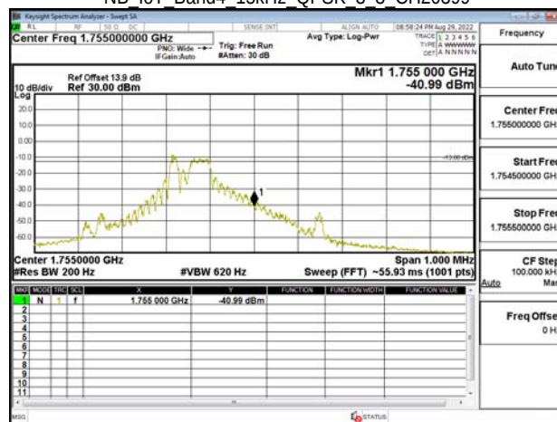
NB IoT Band4 15kHz QPSK 3 3 CH20399
