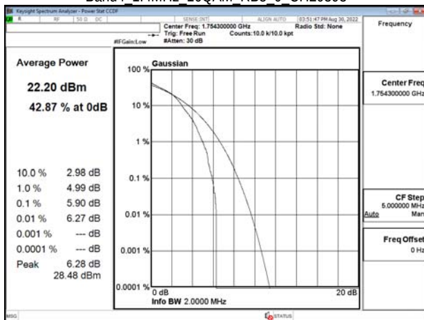
Band4 1.4MHz 16QAM RB5 0 CH20393
