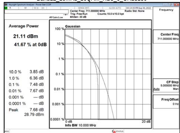
Band12 10MHz 16QAM RB5 0 CH23130
