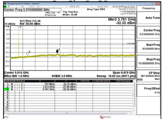
Band12 3MHz QPSK RB1 0 CH23165
