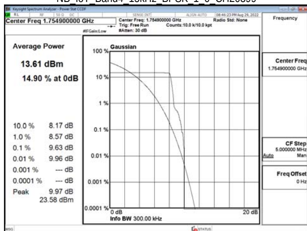
NB IoT Band4 15kHz BPSK 1 0 CH20399
