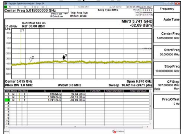
Band12 3MHz QPSK RB1 0 CH23095
