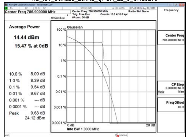
NB IoT Band13 15kHz QPSK 12 0 CH23279
