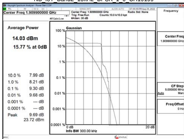
NB IoT Band2 15kHz BPSK 1 0 CH19199
