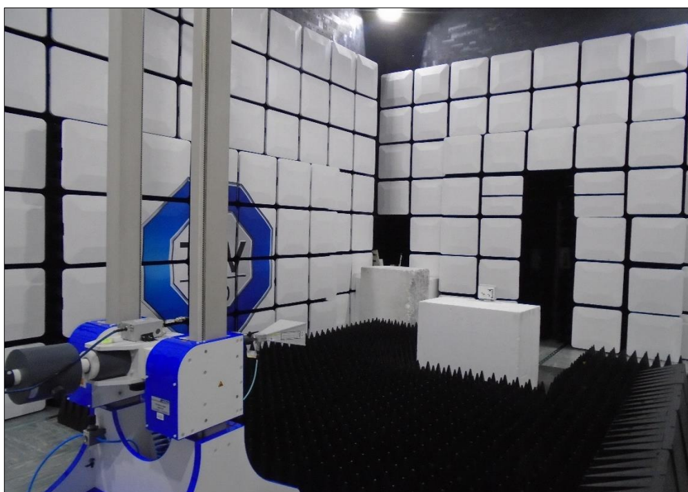
Figure 9 - Test Setup - 1 GHz to 5 GHz
