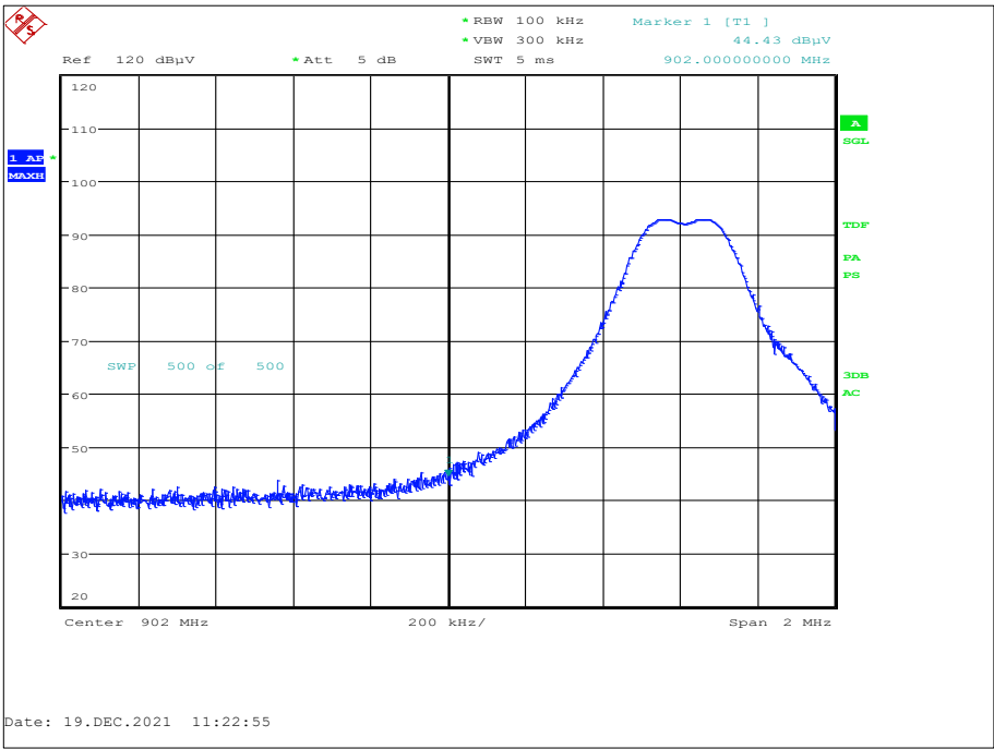
Figure 29 – Authorised Band Edge, 902.6 MHz, Band Edge Frequency: 902.0 MHz
