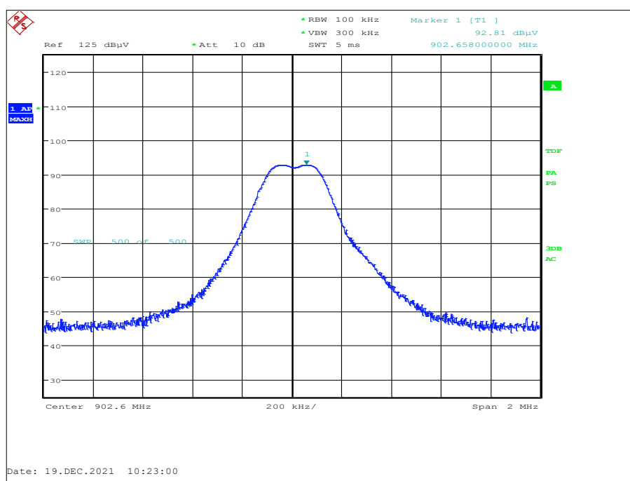
Figure 7 - 902.6 MHz, Peak
