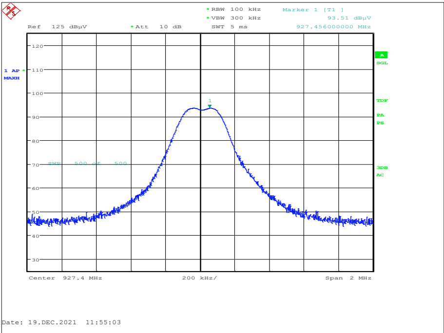
Figure 9 - 927.4 MHz, Peak
