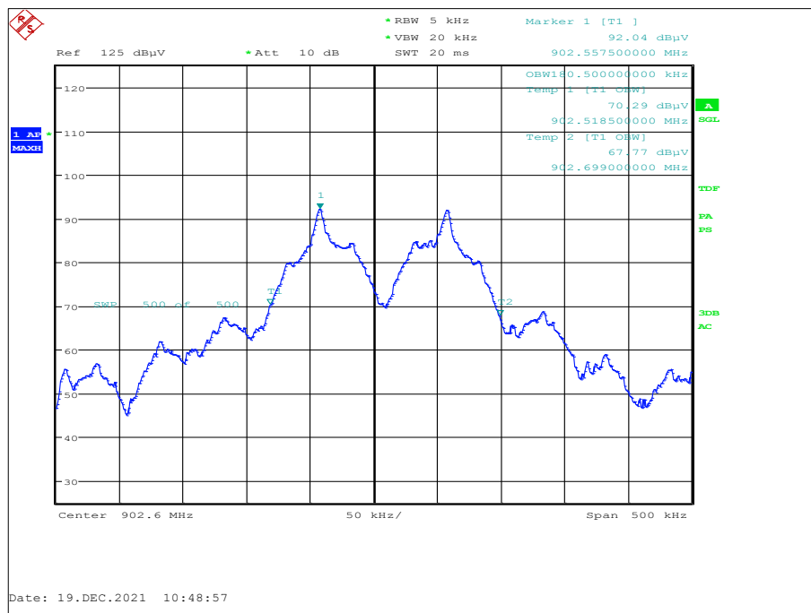
Figure 1 – 902.6 MHz, 99% Occupied Bandwidth
