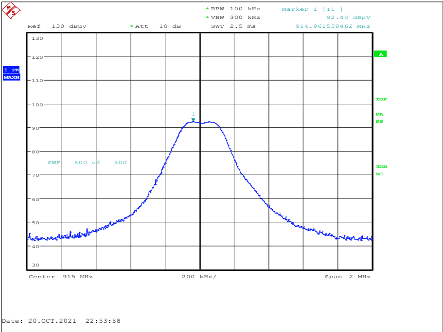
Figure 8 – 915.0 MHz, Peak
