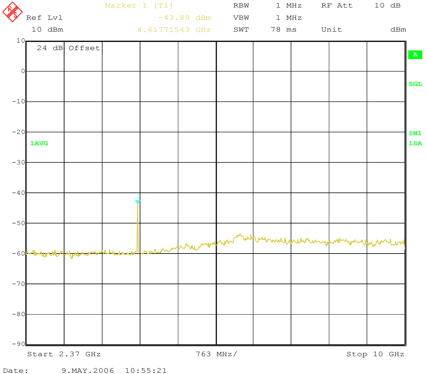
Plot 11 - Spurious emissions at the antenna terminals (2370 MHz to 10 GHz, channel B, 2312.5 MHz)
