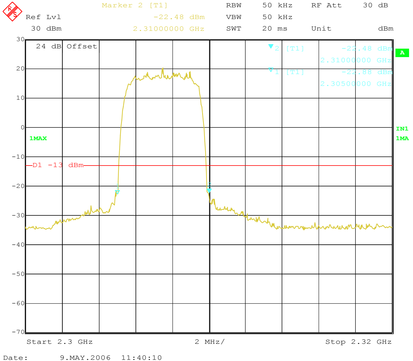
Plot 13 - Spurious emissions (bandedges) at the antenna terminals (2300 MHz to 2320 MHz, channel A, 2307.5 MHz)
