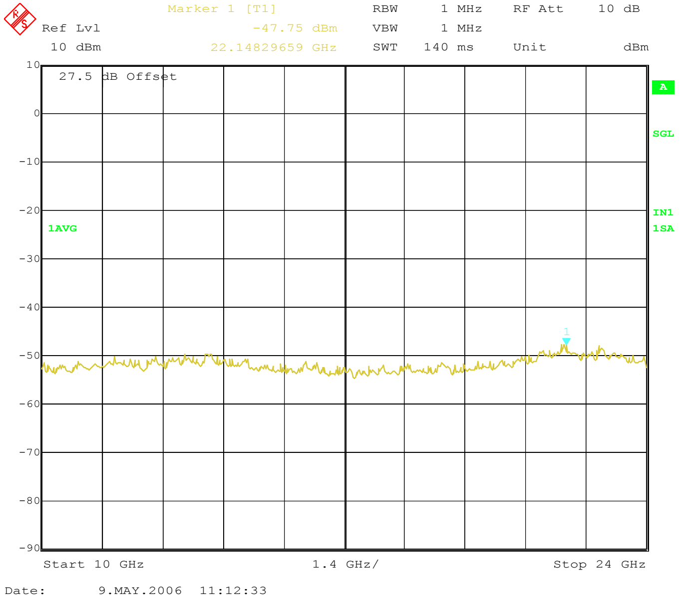
Plot 9 - Spurious emissions at the antenna terminals (10 GHz to 24 GHz, channel A, 2307.5 MHz)
