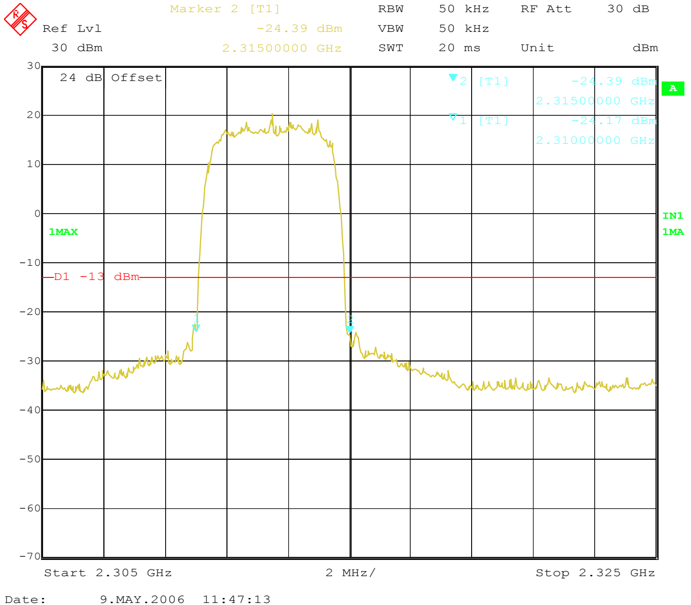
Plot 14 - Spurious emissions (bandedges) at the antenna terminals (2305 MHz to 2325 MHz, channel B, 2312.5 MHz)
