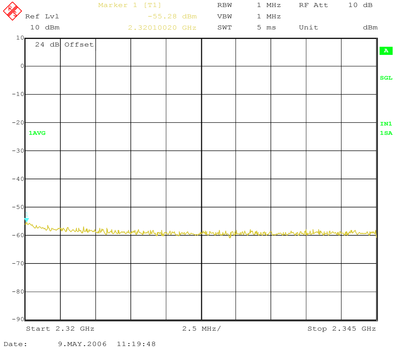
Plot 5 - Spurious emissions at the antenna terminals (2320 MHz to 2345 MHz, channel B, 2312.5 MHz)
