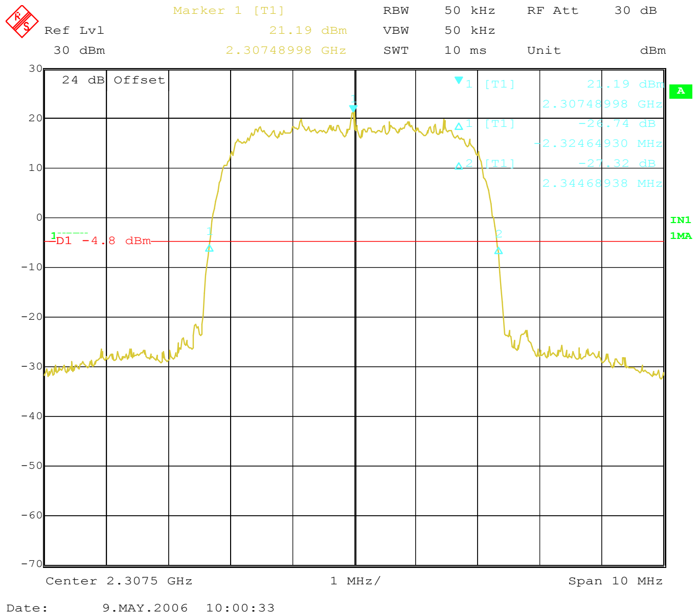
Plot 1 - Occupied bandwidth (-26 dB, channel A, 2307.5 MHz)
