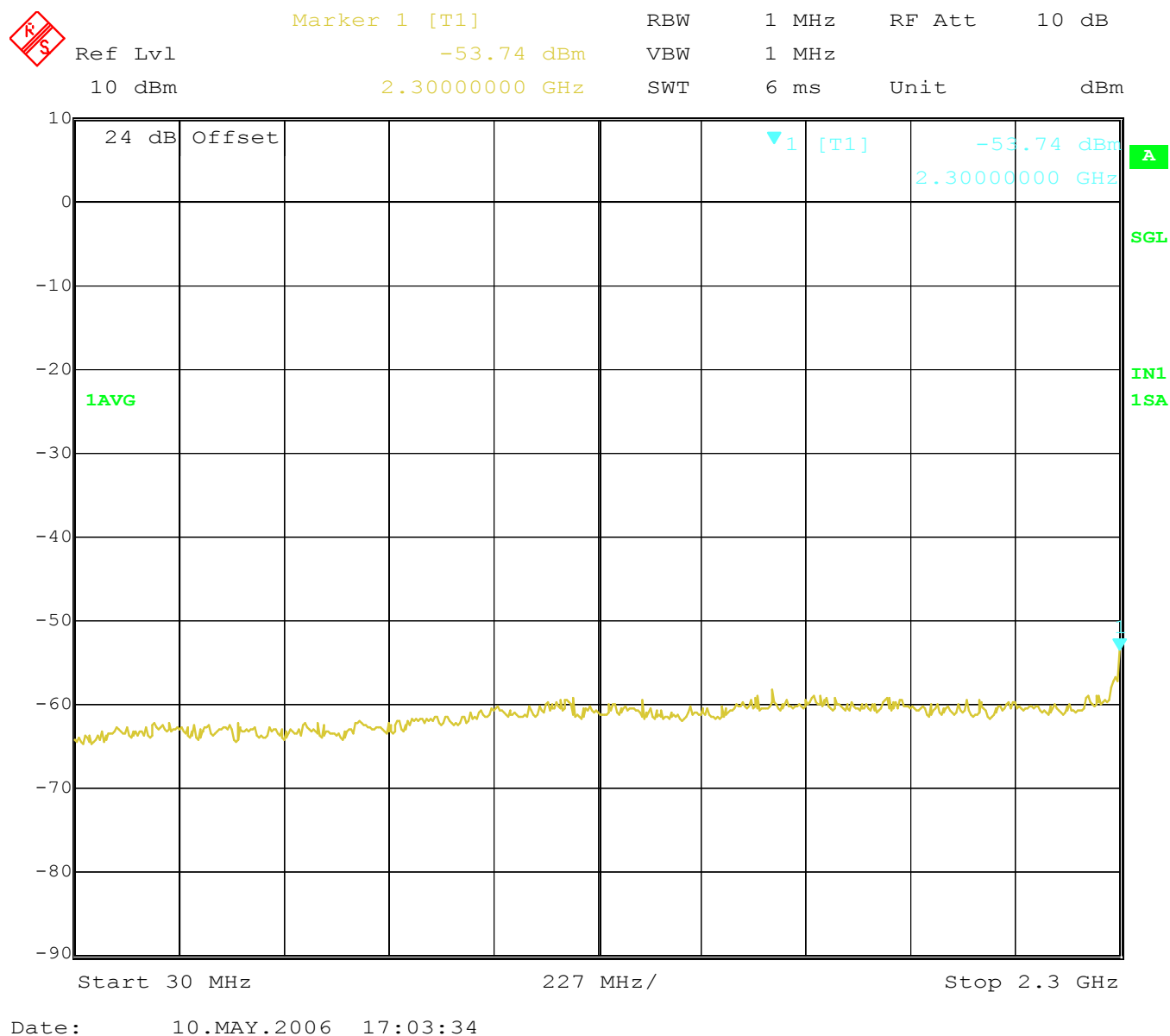
Plot 7 - Spurious emissions at the antenna terminals (30 MHz to 2300 MHz, channel A, 2307.5 MHz)
