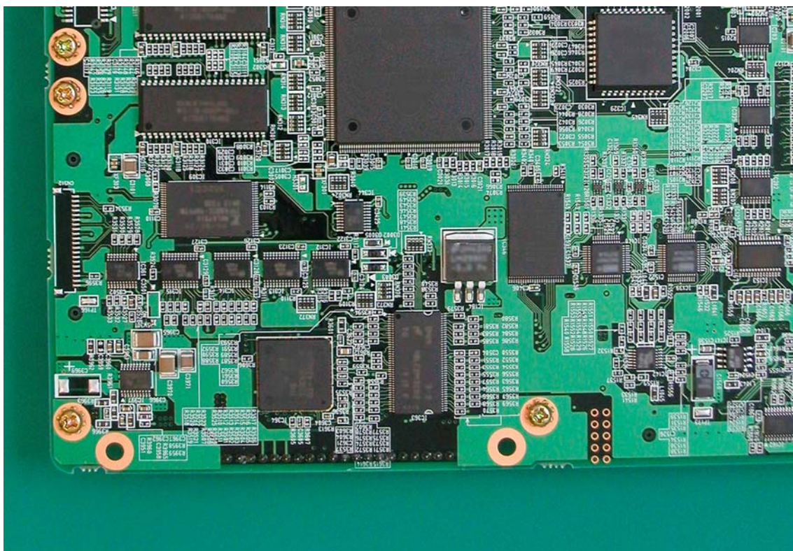
18-2 *Control board –back view (Part 2)
