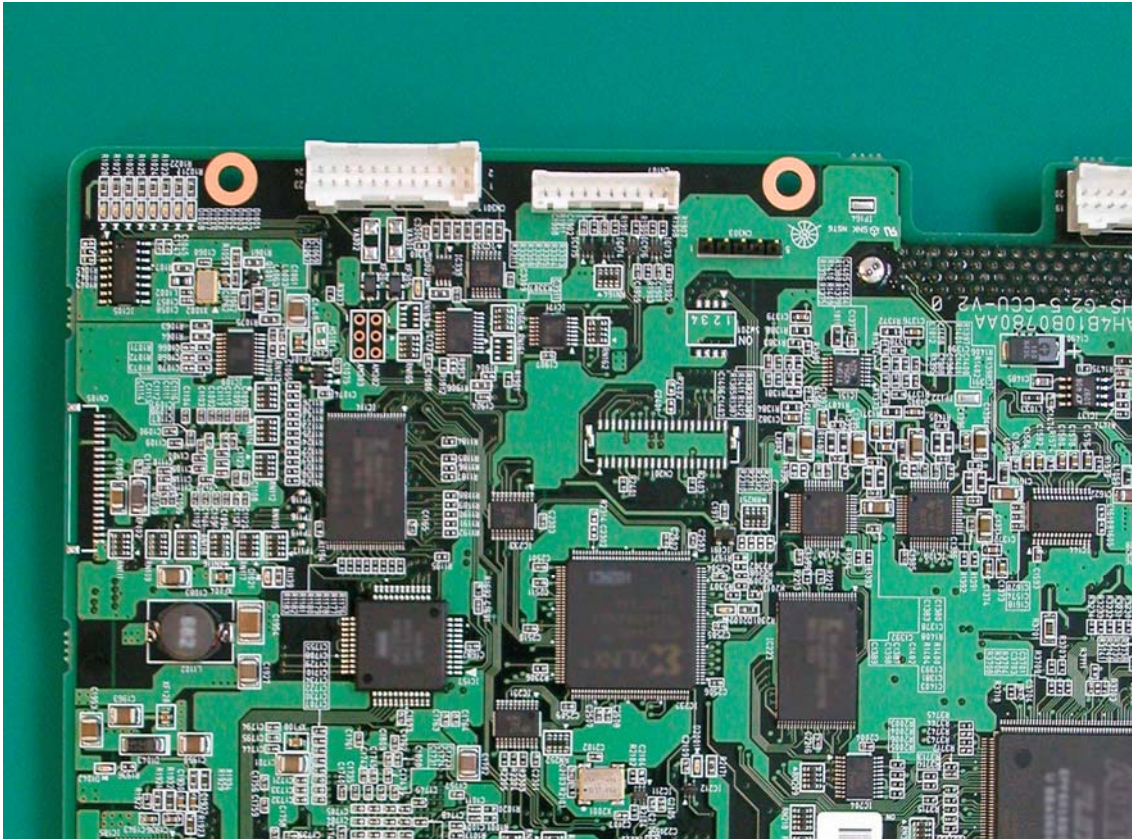
17-1 *Control board –front view (Part 1)
