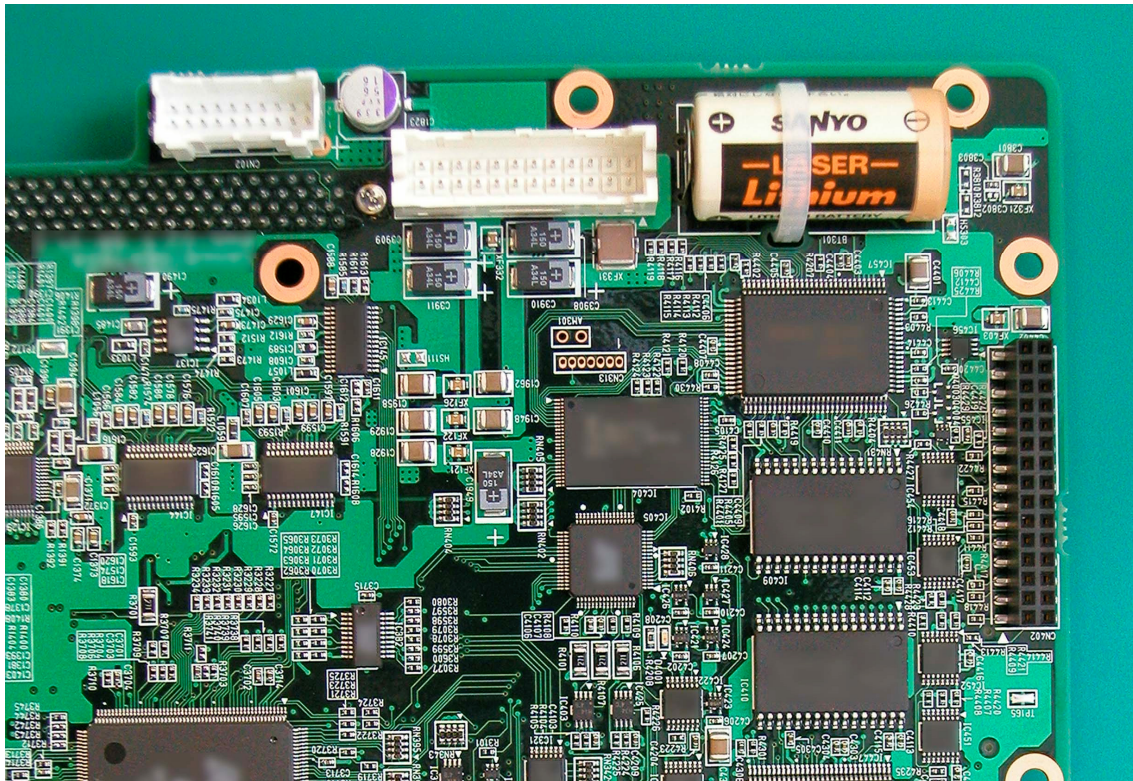
15-3 *Control board –front view (Part 3)
