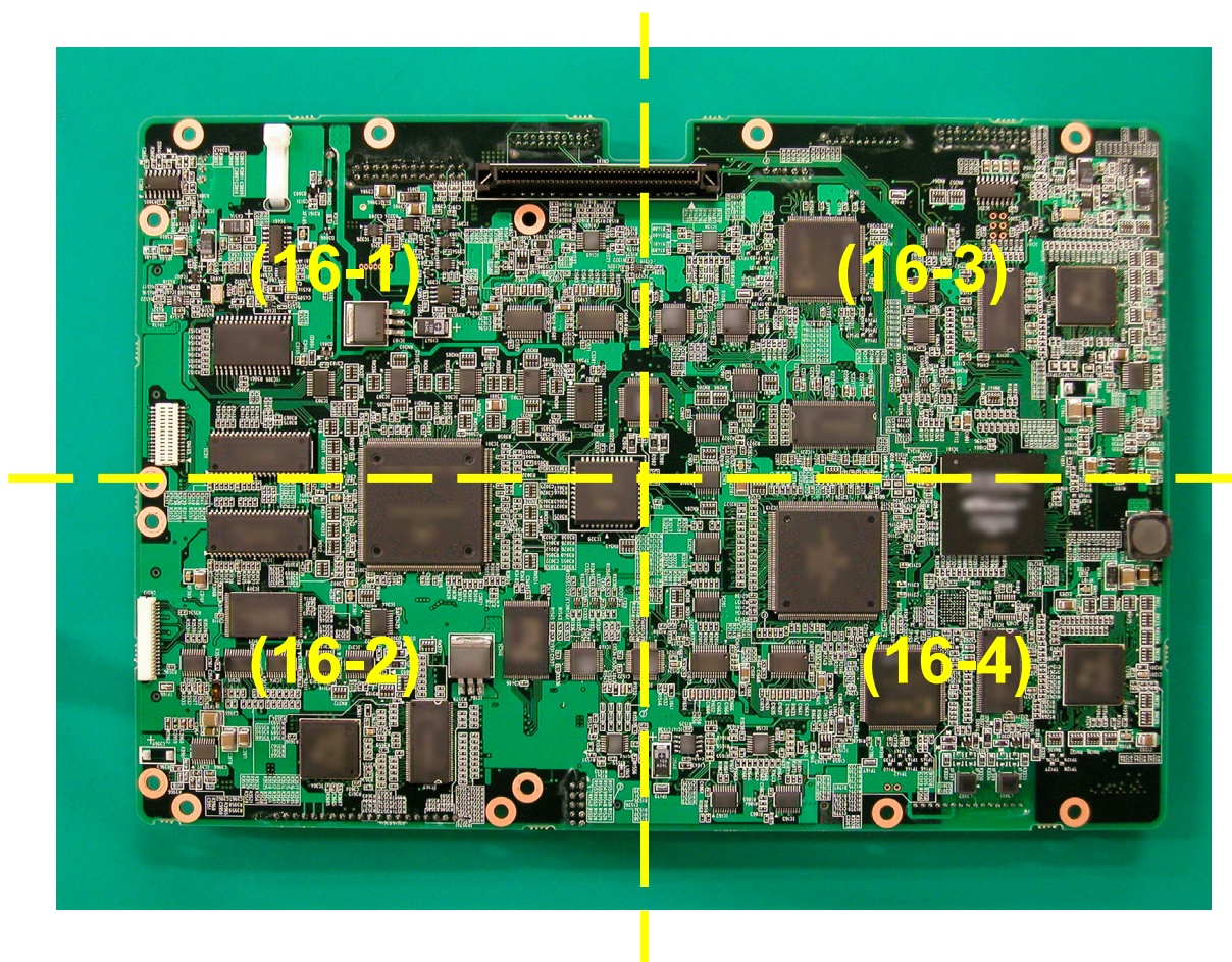
16 Control board (back view)
